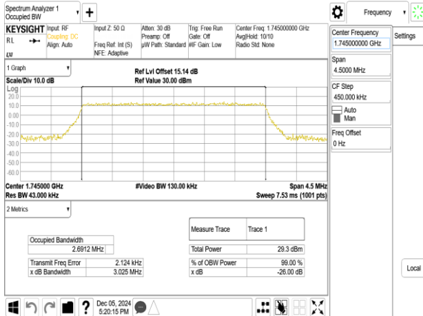
Band66_3MHz_64QAM_RB15_0_CH132322
