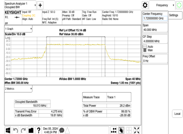
Band66_20MHz_256QAM_RB100_0_CH132072
