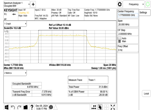
Band66_10MHz_16QAM_RB50_0_CH132622
