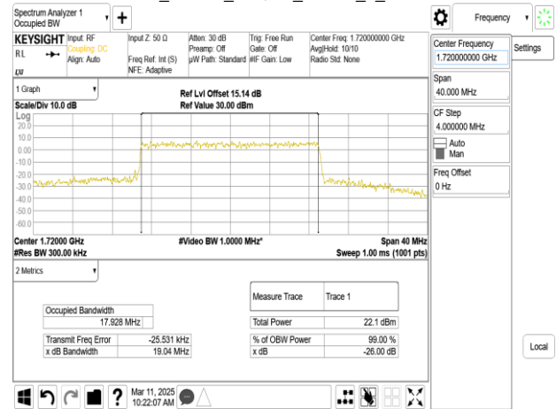
Band66_20MHz_64QAM_RB100_0_CH132072
