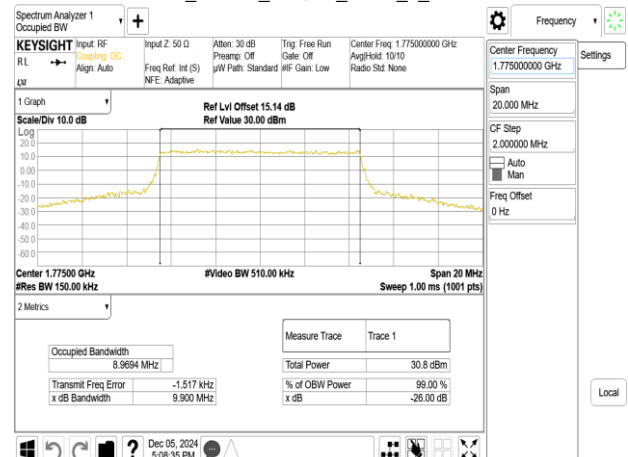
Band66_10MHz_16QAM_RB50_0_CH132622
