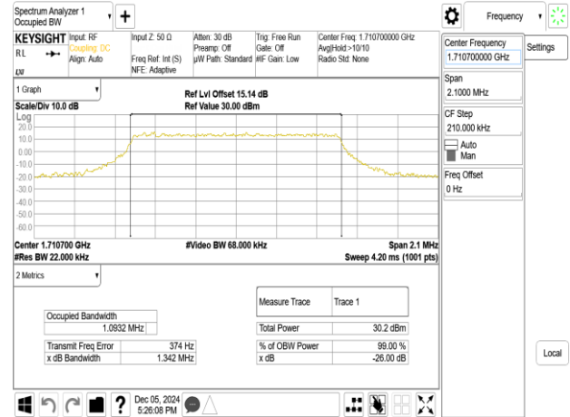
Band66_1.4MHz_64QAM_RB6_0_CH131979
