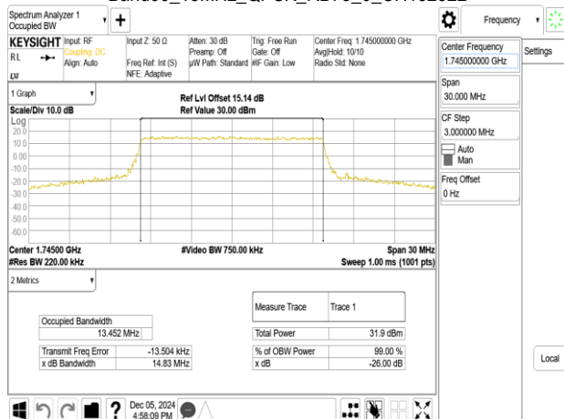
Band66_15MHz_16QAM_RB75_0_CH132322
