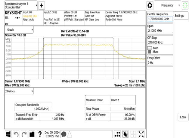
Band66_1.4MHz_16QAM_RB6_0_CH132665
