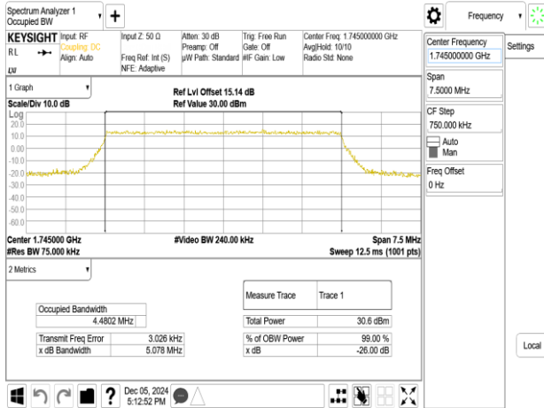
Band66_5MHz_64QAM_RB25_0_CH132322
