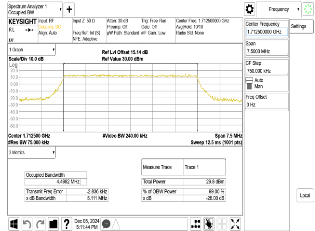
Band66_5MHz_256QAM_RB25_0_CH131997
