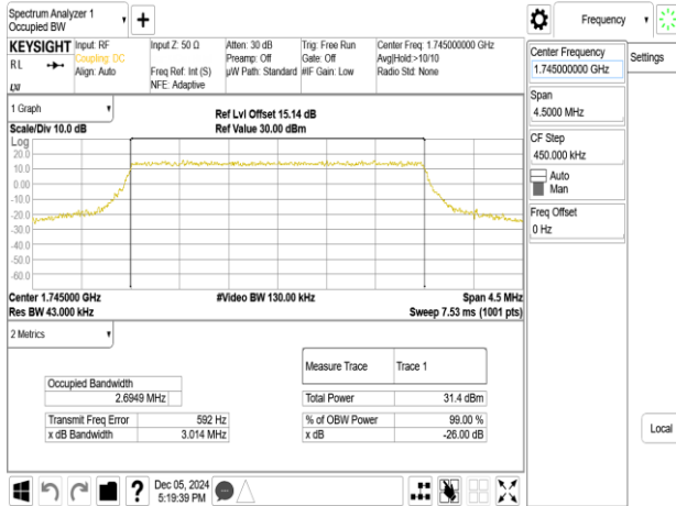
Band66_3MHz_16QAM_RB15_0_CH132322
