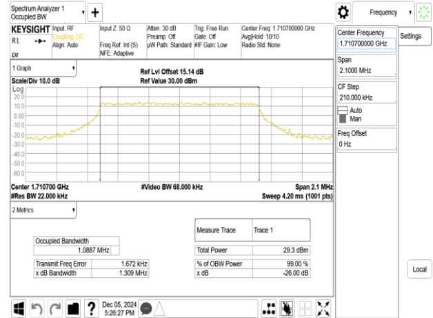
Band66_1.4MHz_256QAM_RB6_0_CH131979
