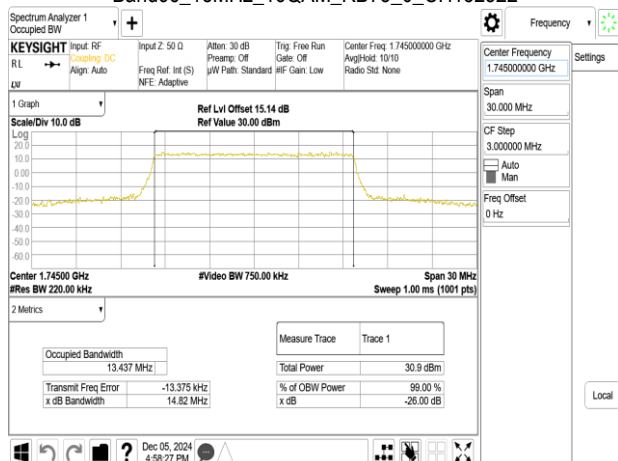
Band66_15MHz_64QAM_RB75_0_CH132322
