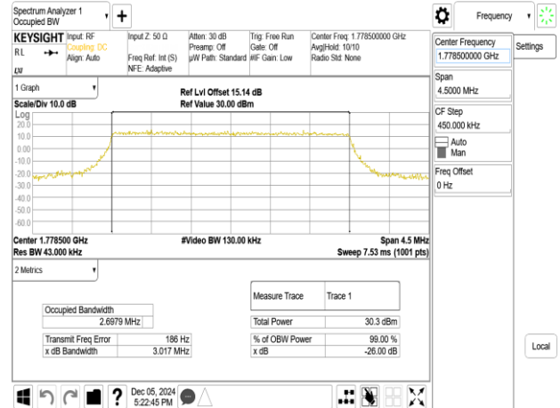
Band66_3MHz_16QAM_RB15_0_CH132657
