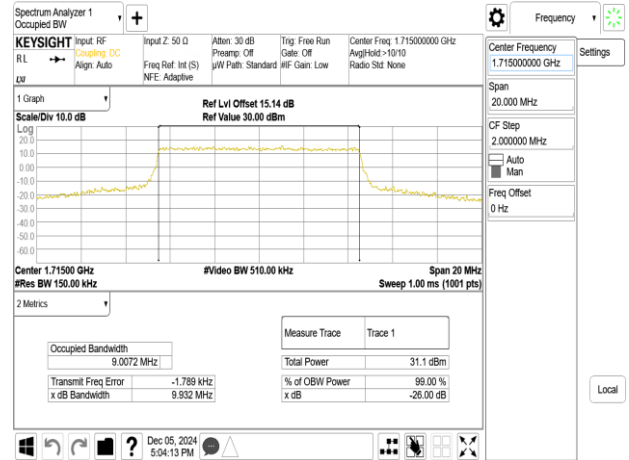
Band66_10MHz_64QAM_RB50_0_CH132022
