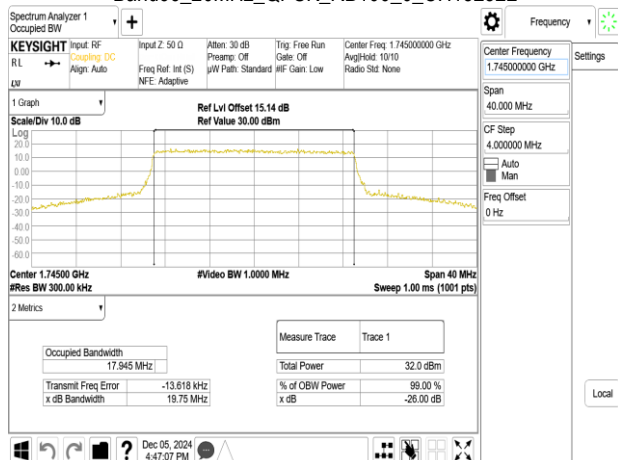
Band66_20MHz_16QAM_RB100_0_CH132322
