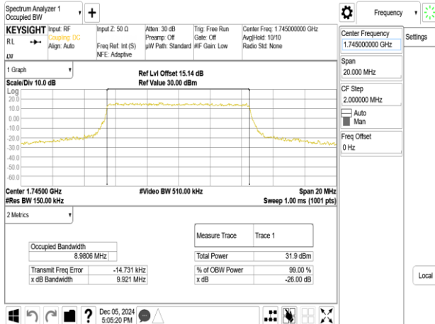
Band66_10MHz_16QAM_RB50_0_CH132322
