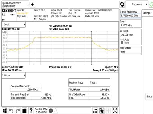
Band66_1.4MHz_256QAM_RB6_0_CH132665
