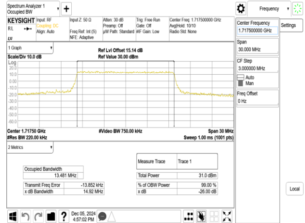
Band66_15MHz_64QAM_RB75_0_CH132047
