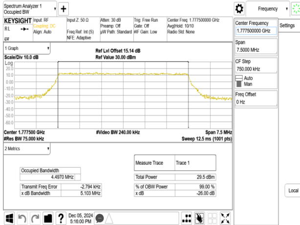
Band66_5MHz_256QAM_RB25_0_CH132647
