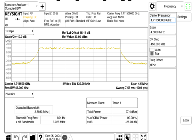
Band66_3MHz_256QAM_RB15_0_CH131987
