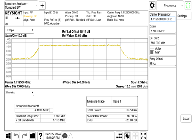
Band66_5MHz_64QAM_RB25_0_CH131997
