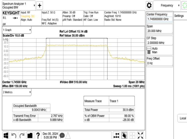
Band66_10MHz_64QAM_RB50_0_CH132322
