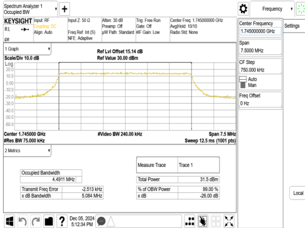
Band66_5MHz_16QAM_RB25_0_CH132322
