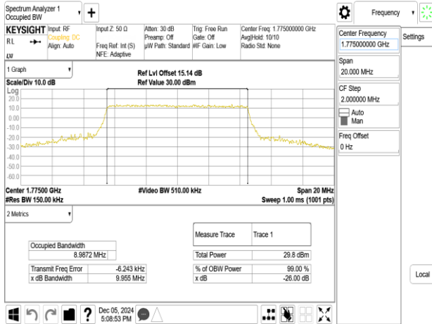
Band66_10MHz_256QAM_RB50_0_CH132622
