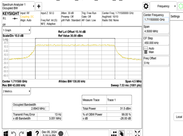
Band66_3MHz_QPSK_RB15_0_CH131987
