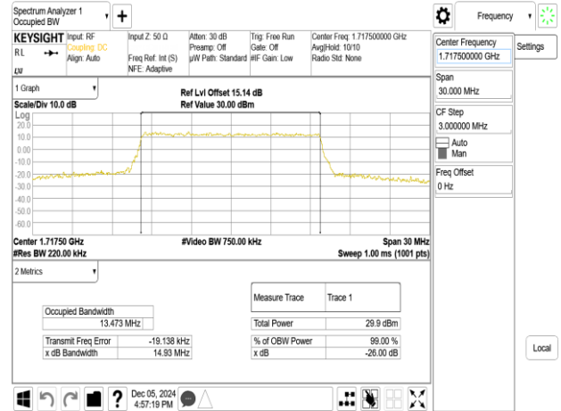
Band66_15MHz_256QAM_RB75_0_CH132047
