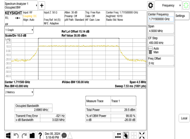
Band66_3MHz_256QAM_RB15_0_CH131987
