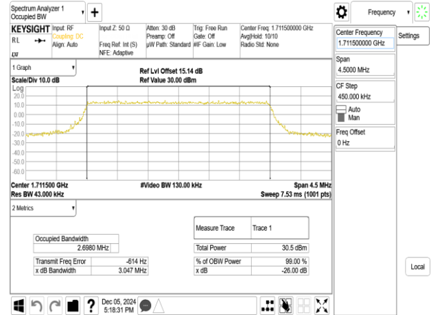
Band66_3MHz_64QAM_RB15_0_CH131987
