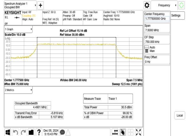
Band66_5MHz_16QAM_RB25_0_CH132647
