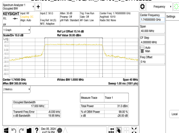
Band66_20MHz_64QAM_RB100_0_CH132322
