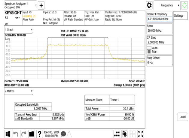
Band66_10MHz_256QAM_RB50_0_CH132022
