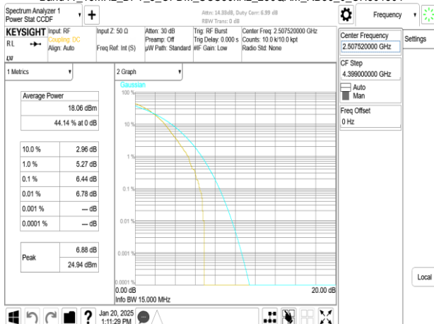
Band41_15MHz_DFT_s_OFDM_SCS30kHz_256QAM_RB36_0_CH501504
