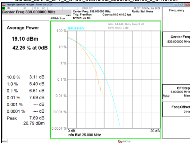
Band26_20MHz_DFT_s_OFDM_SCS15kHz_256QAM_RB100_0_CH167800
