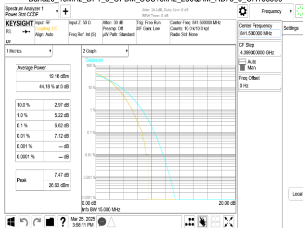
Band26 15MHz_DFT_s_OFDM_SCS15kHz_256QAM_RB75_0_CH168300
