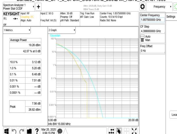
Band25_15MHz_DFT_s_OFDM_SCS15kHz_256QAM_RB75_0_CH371500
