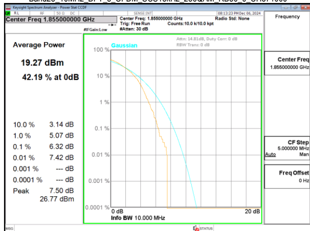
Band25_10MHz_DFT_s_OFDM_SCS15kHz_256QAM_RB50_0_CH371000
