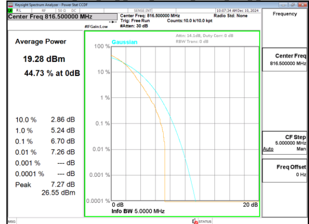
Band26-Part90s_5MHz_DFT_s_OFDM_SCS15kHz_256QAM_RB25_0_CH163300
