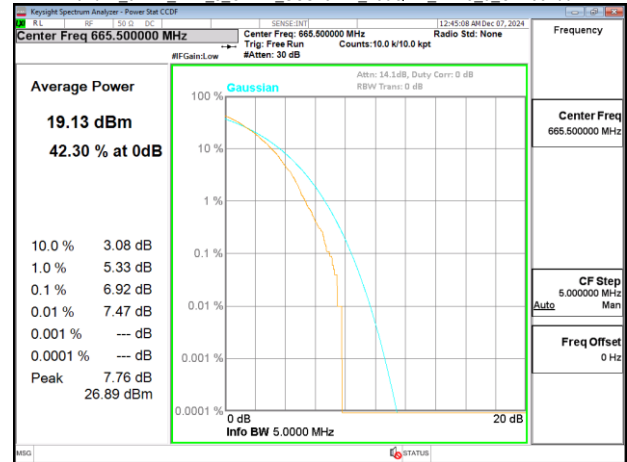
Band71 5MHz DFT s OFDM SCS15kHz 256QAM RB25_0 CH133100
