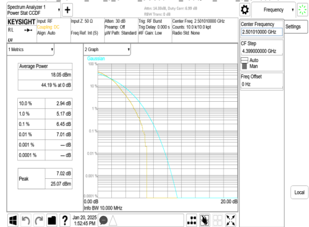
Band41_10MHz_DFT_s_OFDM_SCS30kHz_256QAM_RB24_0_CH501000
