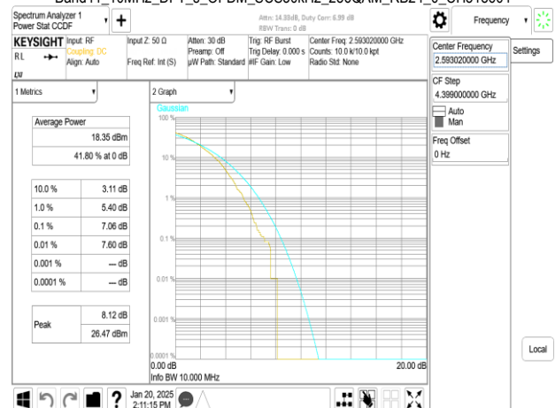
Band41_10MHz_DFT_s_OFDM_SCS30kHz_256QAM_RB24_0_CH518604
