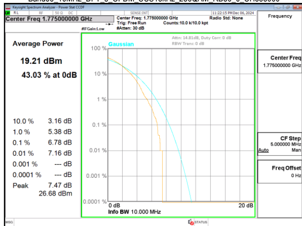
Band66 10MHz_DFT_s_OFDM_SCS15kHz_256QAM_RB50_0_CH355000
