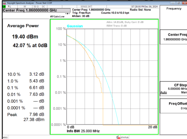
Band25_20MHz_DFT_s_OFDM_SCS15kHz_256QAM_RB100_0_CH372000
