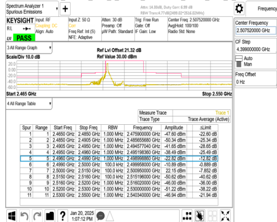
Band41_15MHz_DFT_s_OFDM_SCS30kHz_BPSK_RB1_0_CH501504
