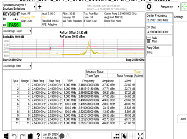
Band41_20MHz_DFT_s_OFDM_SCS30kHz_BPSK_RB50_0_CH502002
