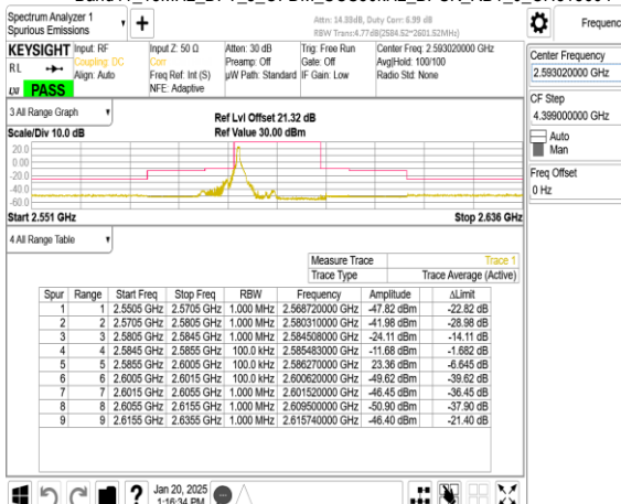
Band41_15MHz_DFT_s_OFDM_SCS30kHz_BPSK_RB1_0_CH518604
