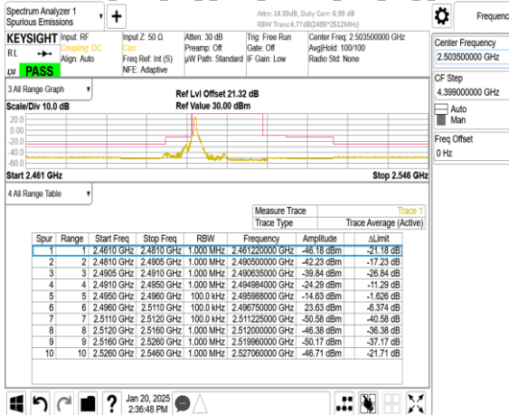
Band41_15MHz_DFT_s_OFDM_SCS30kHz_BPSK_RB1_0_CH500700
