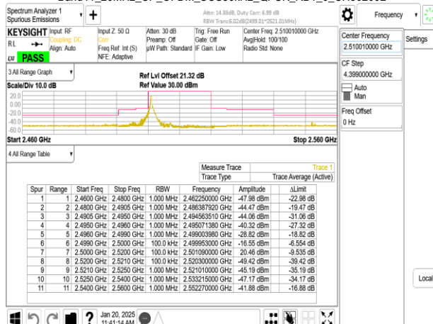
Band41_20MHz_CP_OFDM_SCS30kHz_QPSK_RB1_0_CH502002
