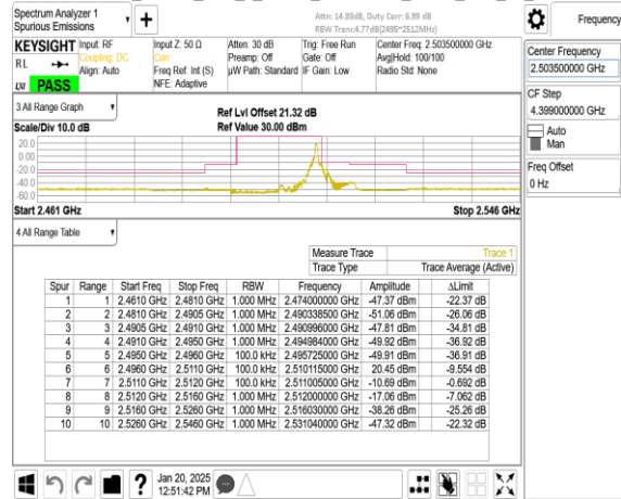
Band41_15MHz_DFT_s_OFDM_SCS30kHz_BPSK_RB36_0_CH500700
