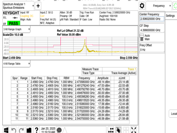
Band41_20MHz_CP_OFDM_SCS30kHz_QPSK_RB51_0_CH501204
