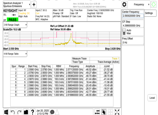
Band41_10MHz_CP_OFDM_SCS30kHz_QPSK_RB24_0_CH518604
