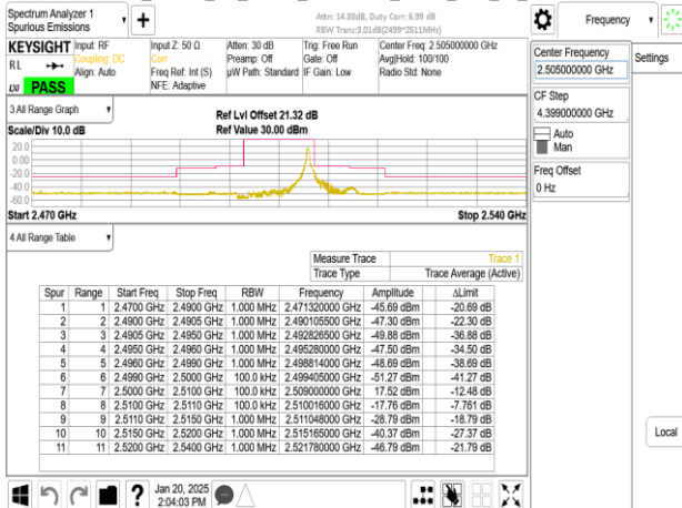
Band41_10MHz_CP_OFDM_SCS30kHz_QPSK_RB24_0_CH501000
