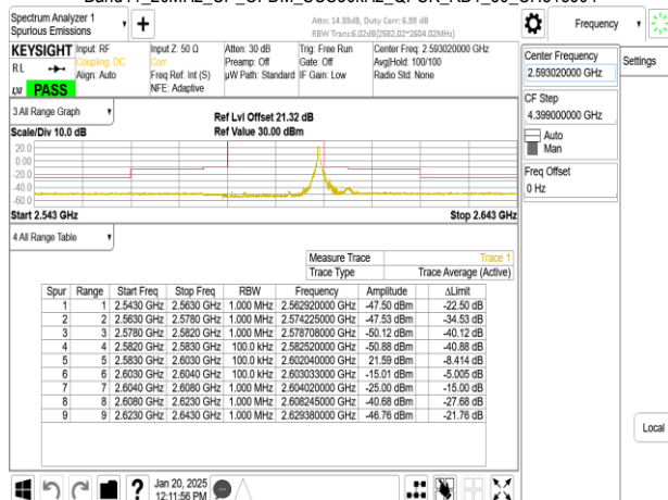
Band41_20MHz_CP_OFDM_SCS30kHz_QPSK_RB51_0_CH518604
