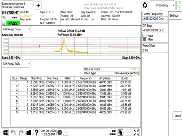
Band41_15MHz_CP_OFDM_SCS30kHz_QPSK_RB1_37_CH518604
