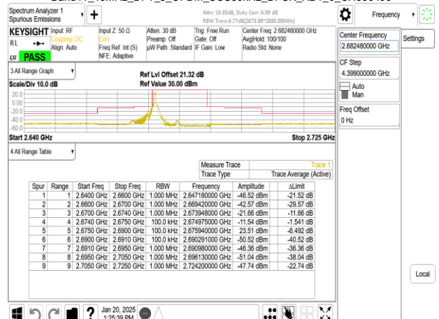
Band41_15MHz_DFT_s_OFDM_SCS30kHz_BPSK_RB1_0_CH536496
