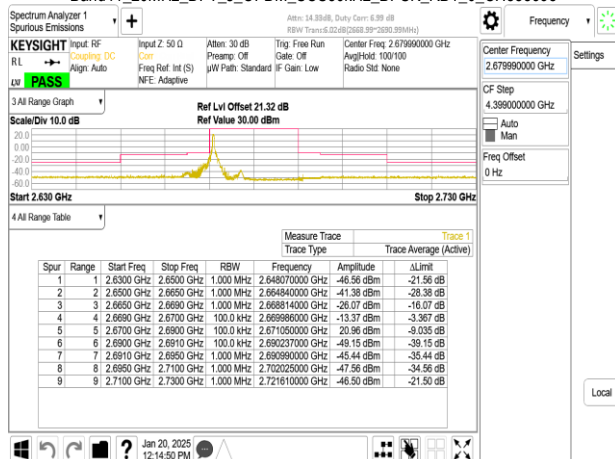
Band41_20MHz_DFT_s_OFDM_SCS30kHz_BPSK_RB1_0_CH535998
