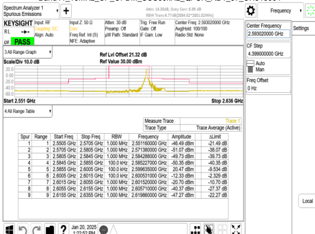
Band41_15MHz_CP_OFDM_SCS30kHz_QPSK_RB1_37_CH518604
