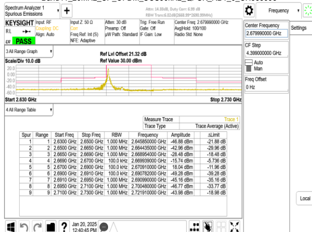
Band41_20MHz_CP_OFDM_SCS30kHz_QPSK_RB1_0_CH535998
