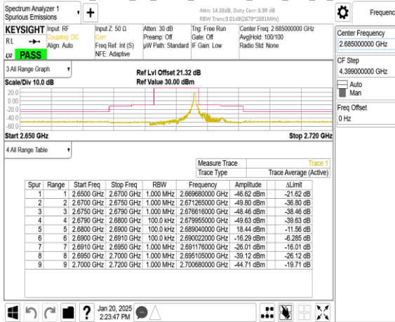
Band41_10MHz_CP_OFDM_SCS30kHz_QPSK_RB24_0_CH537000
