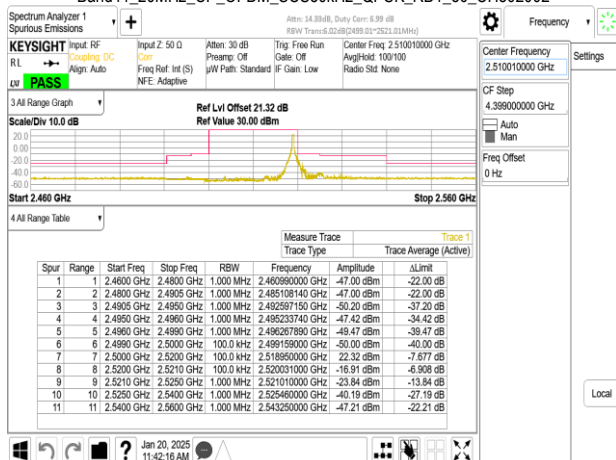
Band41_20MHz_CP_OFDM_SCS30kHz_QPSK_RB51_0_CH502002
