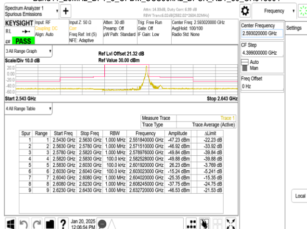
Band41_20MHz_DFT_s_OFDM_SCS30kHz_BPSK_RB50_0_CH518604
