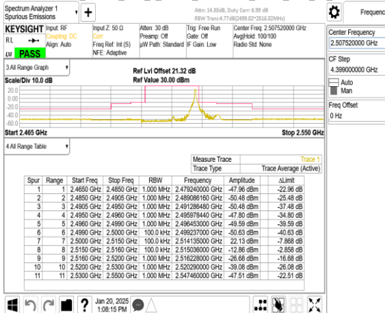
Band41_15MHz_DFT_s_OFDM_SCS30kHz_BPSK_RB36_0_CH501504
