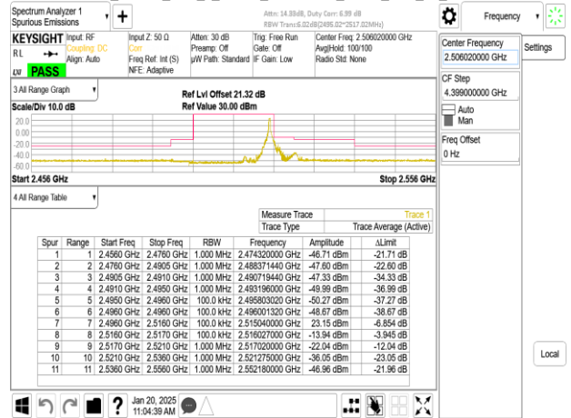
Band41_20MHz_DFT_s_OFDM_SCS30kHz_BPSK_RB50_0_CH501204
