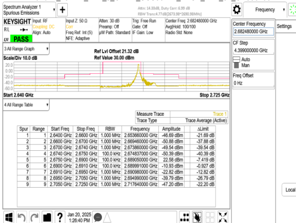
Band41_15MHz_DFT_s_OFDM_SCS30kHz_BPSK_RB36_0_CH536496
