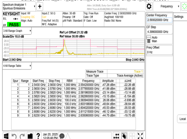
Band41_20MHz_DFT_s_OFDM_SCS30kHz_BPSK_RB1_0_CH518604
