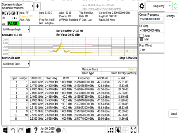
Band41_20MHz_DFT_s_OFDM_SCS30kHz_BPSK_RB1_0_CH501204
