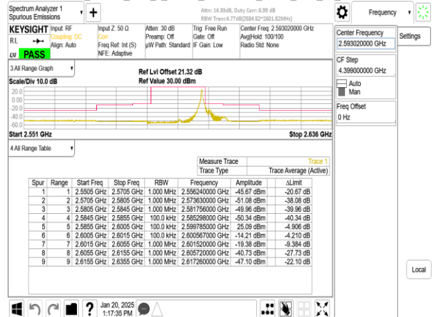
Band41_15MHz_DFT_s_OFDM_SCS30kHz_BPSK_RB36_0_CH518604
