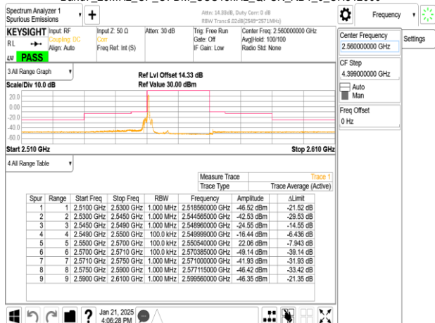
Band7_20MHz_CP_OFDM_SCS15kHz_QPSK_RB1_0_CH512000
