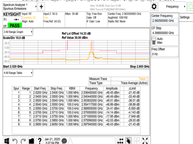
Band7_15MHz_DFT_s_OFDM_SCS15kHz_BPSK_RB1_78_CH512500
