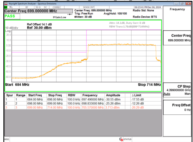
Band12_15MHz_DFT_s_OFDM_SCS15kHz_BPSK_RB1_78_CH141700
