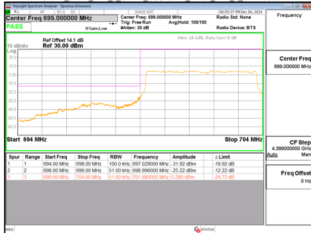
Band12_5MHz_DFT_s_OFDM_SCS15kHz_BPSK_RB25_0_CH140300
