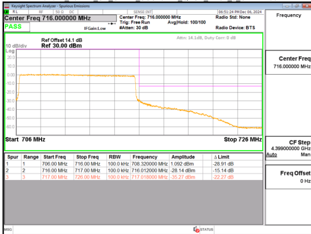
Band12_15MHz_DFT_s_OFDM_SCS15kHz_BPSK_RB1_0_CH141300
