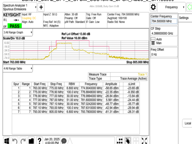
Band13_5MHz_DFT_s_OFDM_SCS15kHz_BPSK_RB25_0_CH155900
