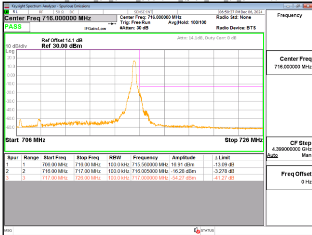
Band12_10MHz_CP_OFDM_SCS15kHz_QPSK_RB52_0_CH142200
