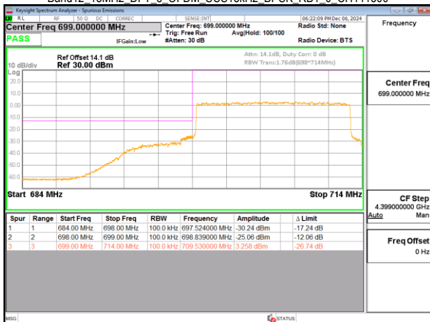
Band12_15MHz_DFT_s_OFDM_SCS15kHz_BPSK_RB1_0_CH141300
