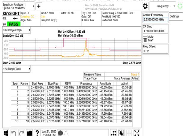
Band7_15MHz_DFT_s_OFDM_SCS15kHz_BPSK_RB1_78_CH507000
