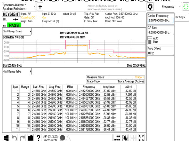
Band7_15MHz_DFT_s_OFDM_SCS15kHz_BPSK_RB1_0_CH507000
