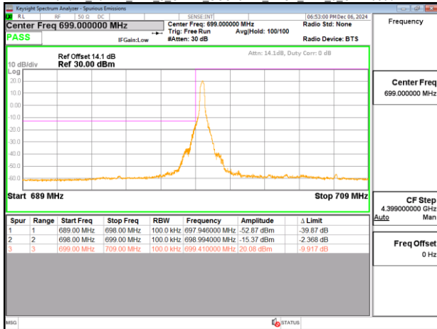
Band12_10MHz_DFT_s_OFDM_SCS15kHz_BPSK_RB50_0_CH140800
