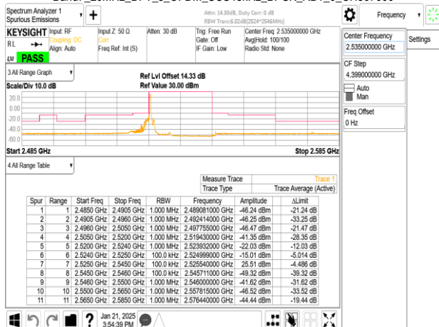
Band7_20MHz_DFT_s_OFDM_SCS15kHz_BPSK_RB1_0_CH507000
