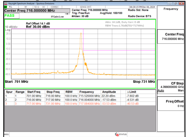
Band12_15MHz_DFT_s_OFDM_SCS15kHz_BPSK_RB75_0_CH141700
