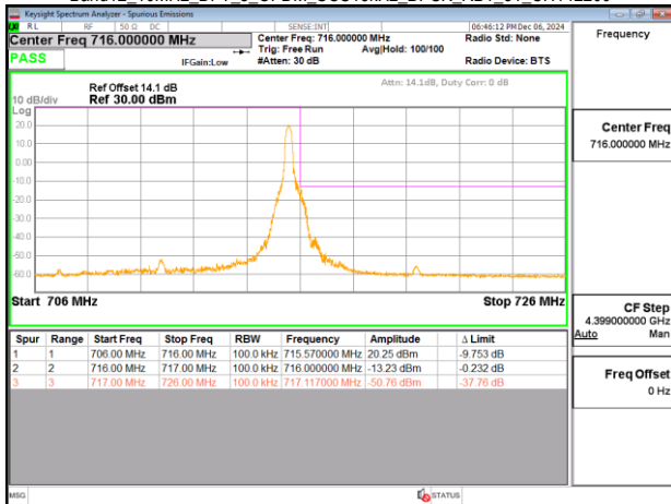
Band12_10MHz_DFT_s_OFDM_SCS15kHz_BPSK_RB1_51_CH142200
