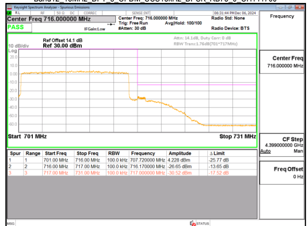
Band12_15MHz_DFT_s_OFDM_SCS15kHz_BPSK_RB75_0_CH141700
