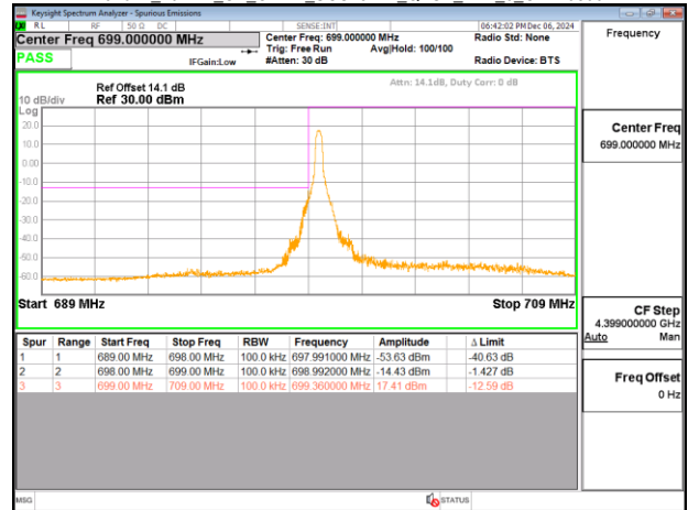
Band12_10MHz_CP_OFDM_SCS15kHz_QPSK_RB52_0_CH140800
