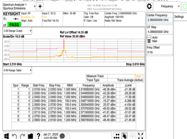
Band7_20MHz_DFT_s_OFDM_SCS15kHz_BPSK_RB1_0_CH512000
