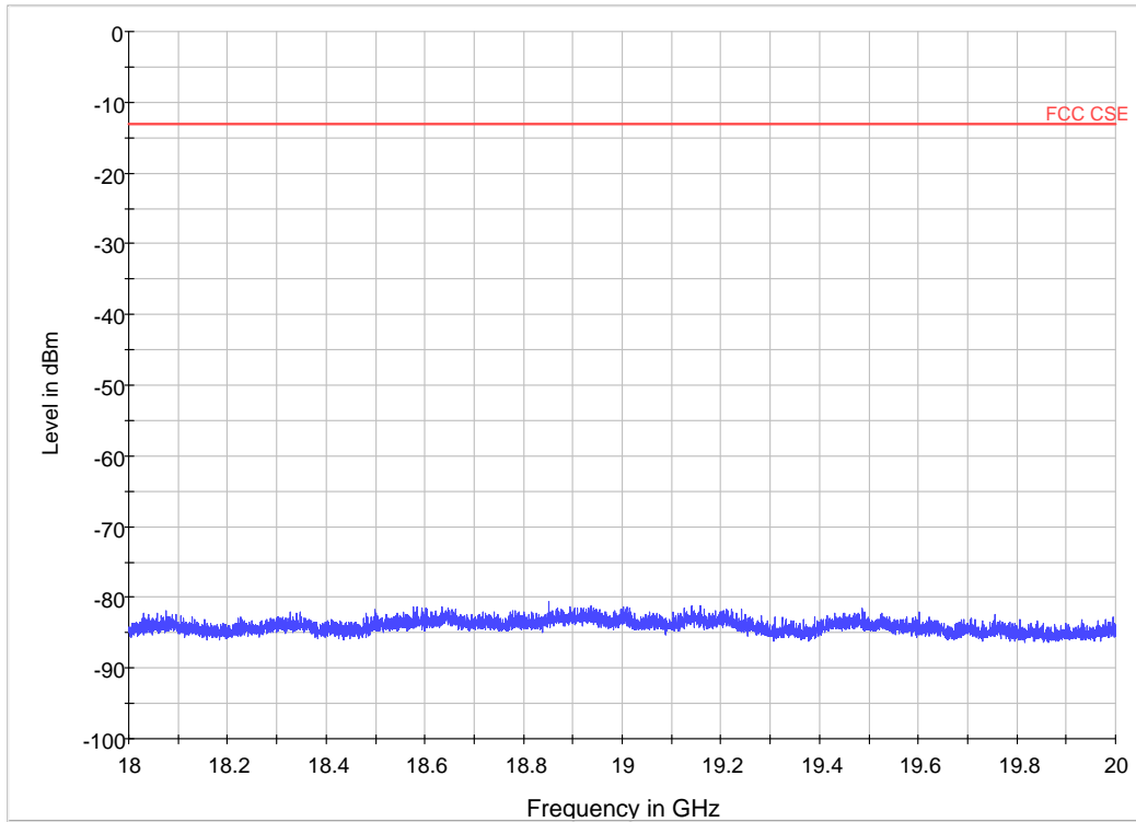
WCDMA Band II CH9262 Channel 18GHz~20GHz
