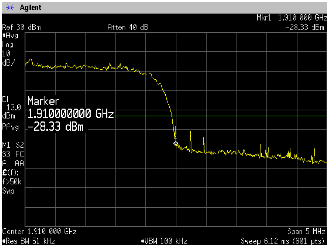
WCDMA Band II HSUPA CH9538 Channel
