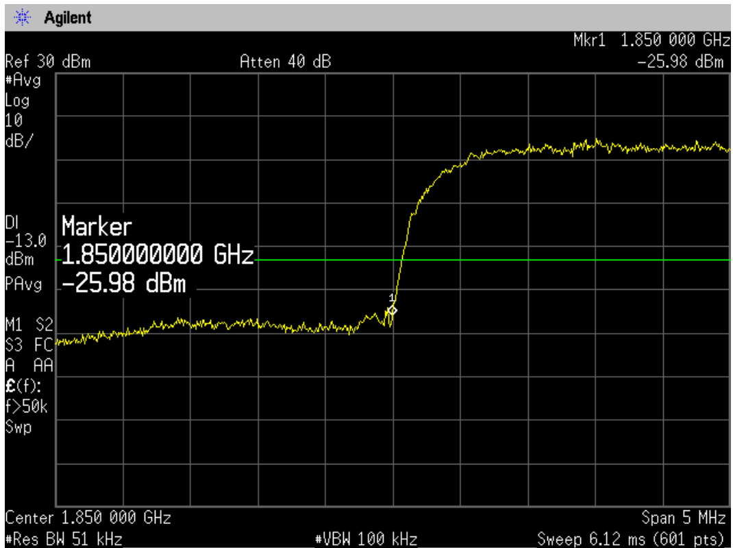
WCDMA Band II HSDPA CH9262 Channel
