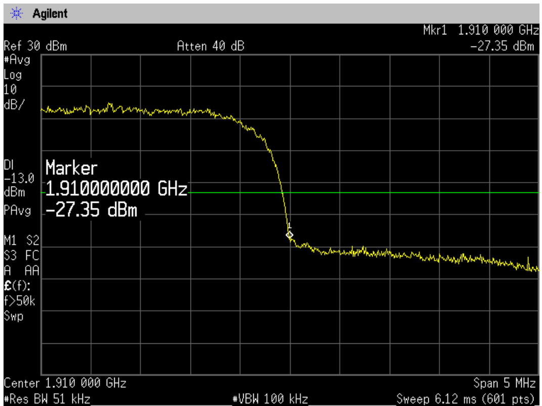
WCDMA Band II HSDPA CH9538 Channel
