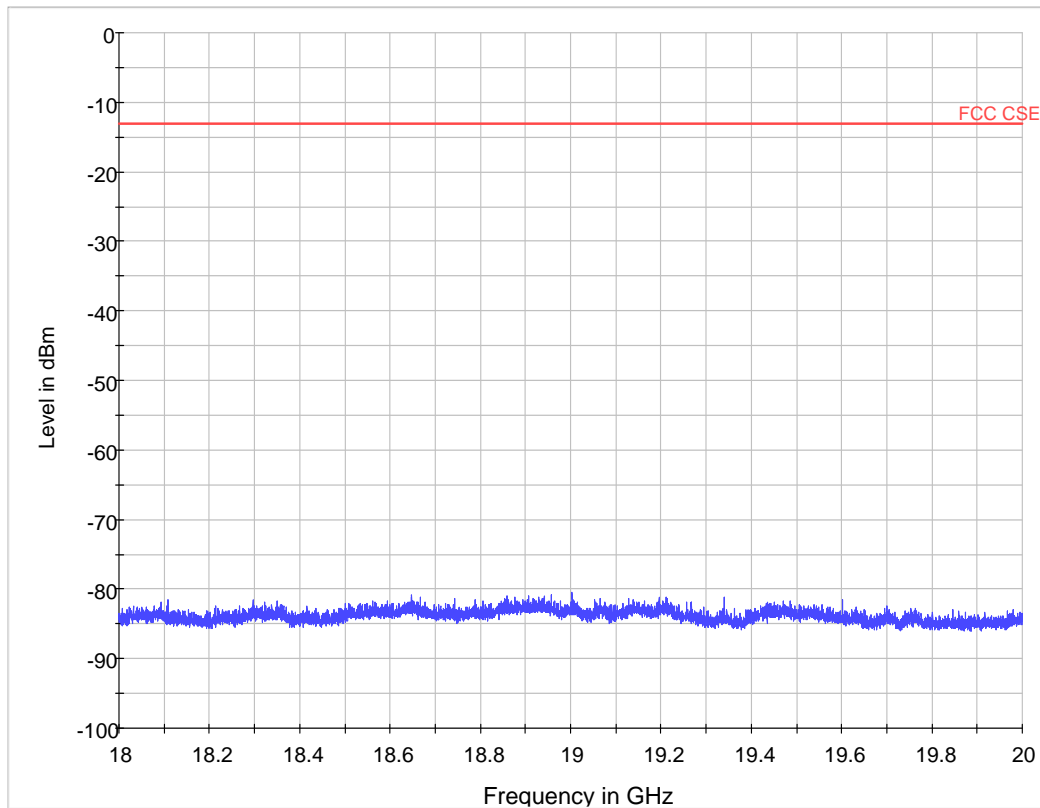
WCDMA Band II CH9538 Channel 18GHz~20GHz
