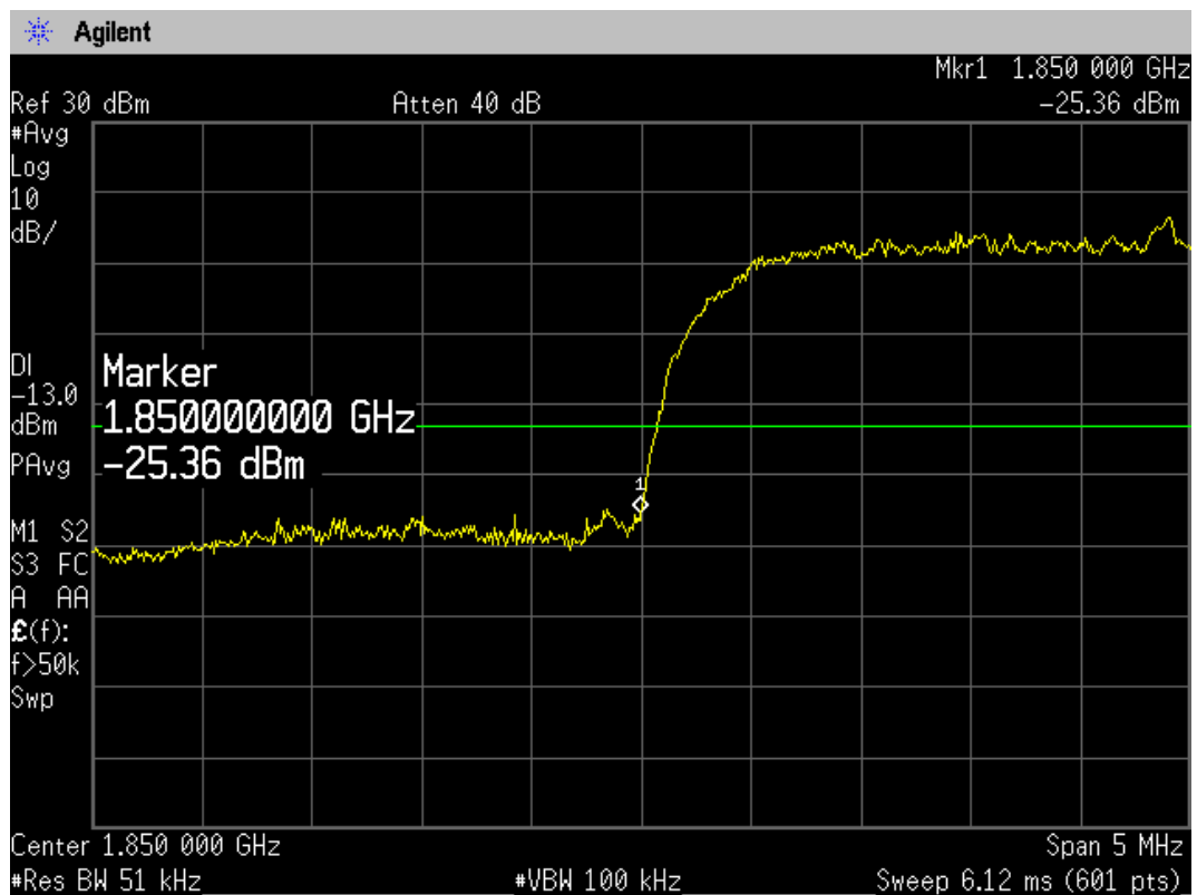
WCDMA Band II CH9262 Channel
