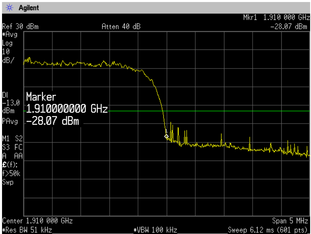
WCDMA Band II CH9538 Channel
