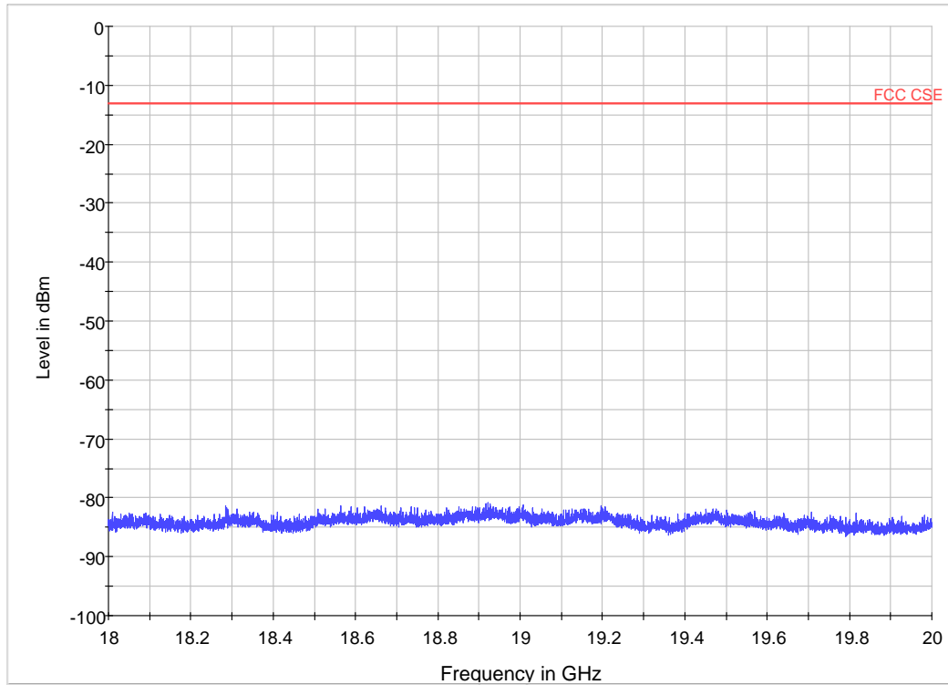
WCDMA Band II CH9400 Channel 18GHz~20GHz
