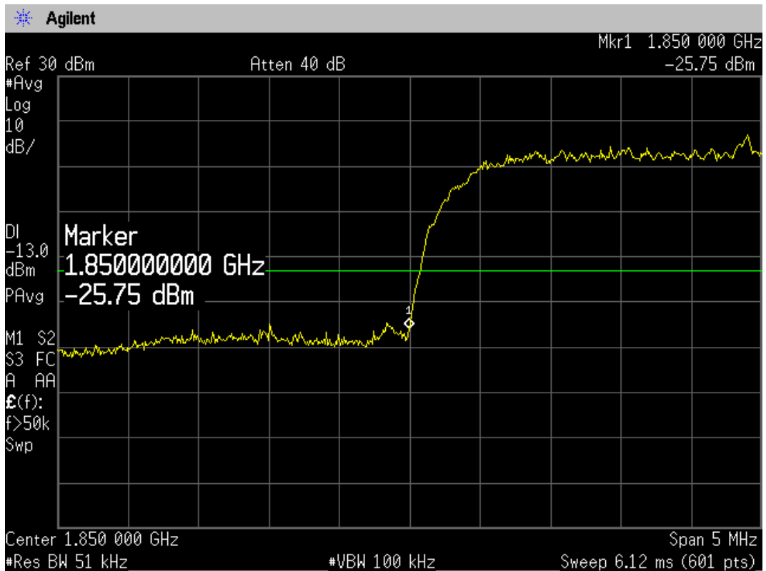
WCDMA Band II HSUPA CH9262 Channel
