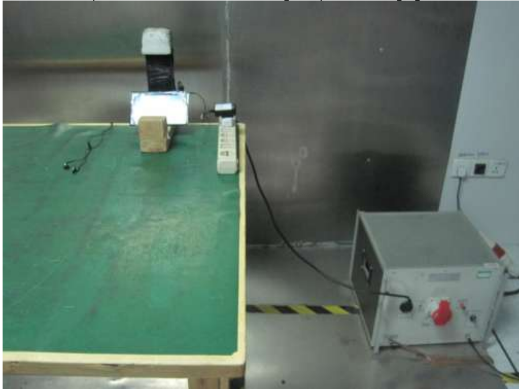
Setup of the worst mode: Wifi Linking+Earphone+Charging Mode
