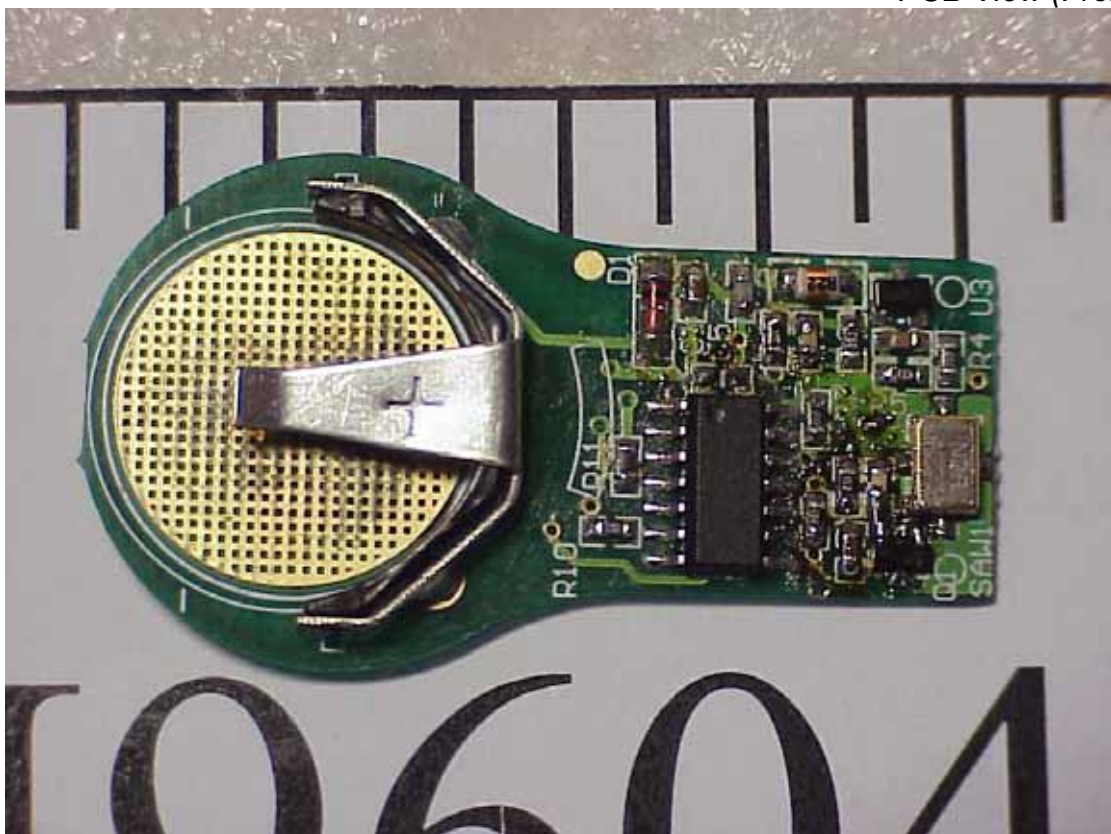
Photos 4 PCB View (Front Side)
