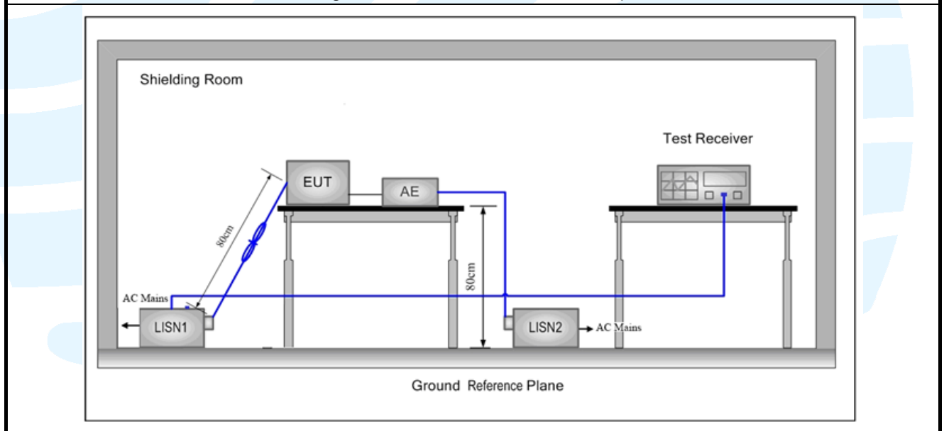
Figure 3. Conducted Emissions setup
