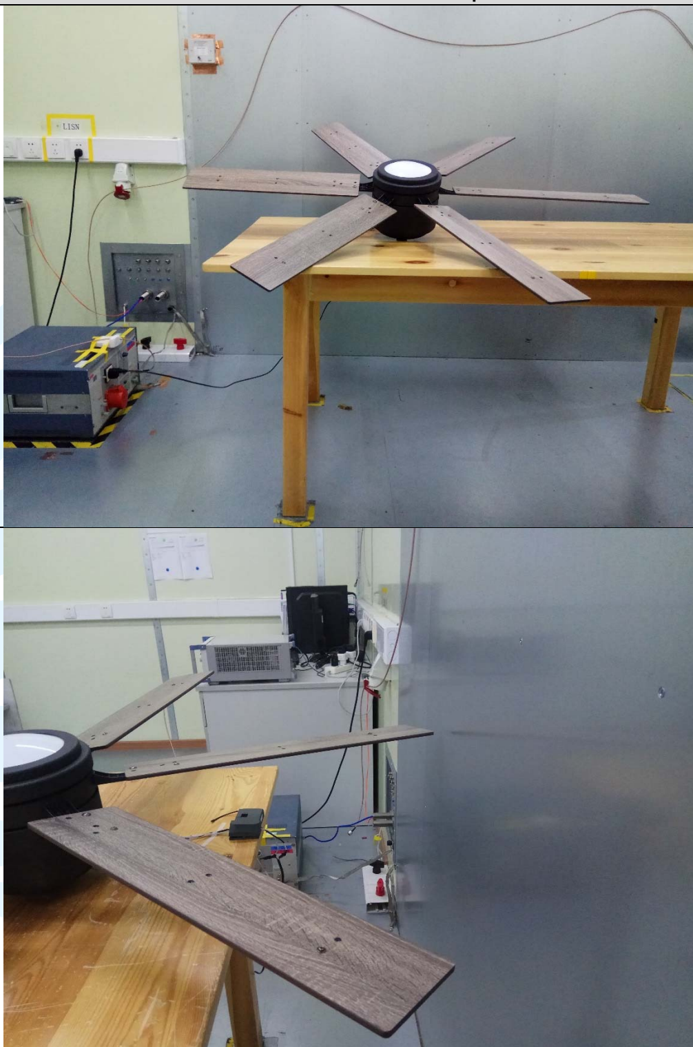
Conducted Emission Test Setup-3
