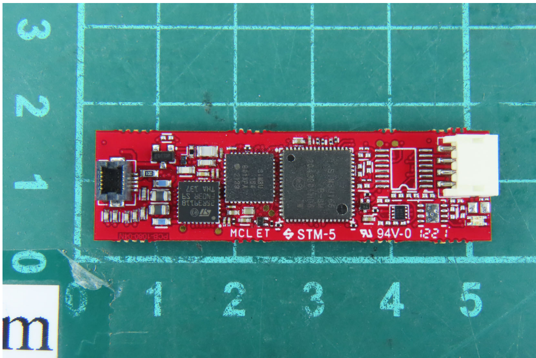
(79) EUT Photo
