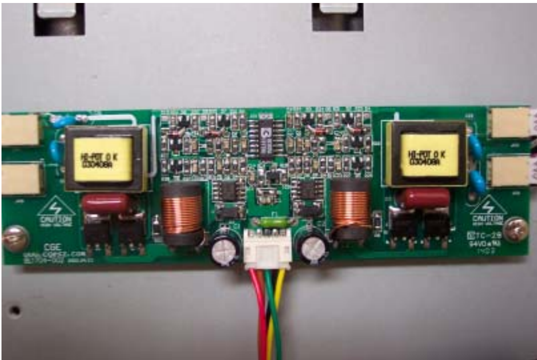
(Inverter)
