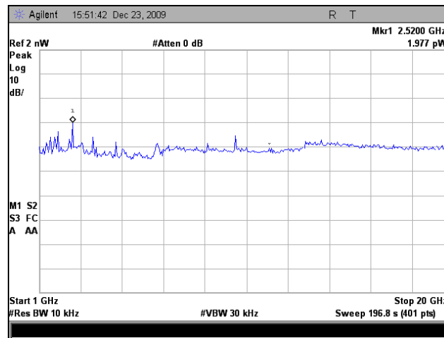
Plot 270. Conducted Receiver Spurious Emissions, Port 2, 1 GHz – 20 GHz
