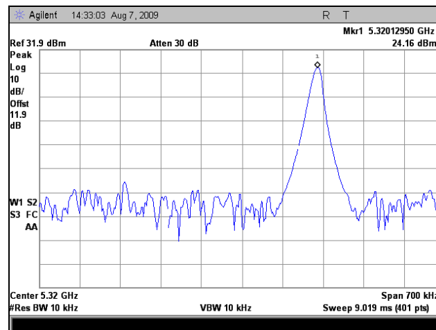
Plot 261. Freq. Stability, Port 3, 5320 MHz @+60C Low Volt.
