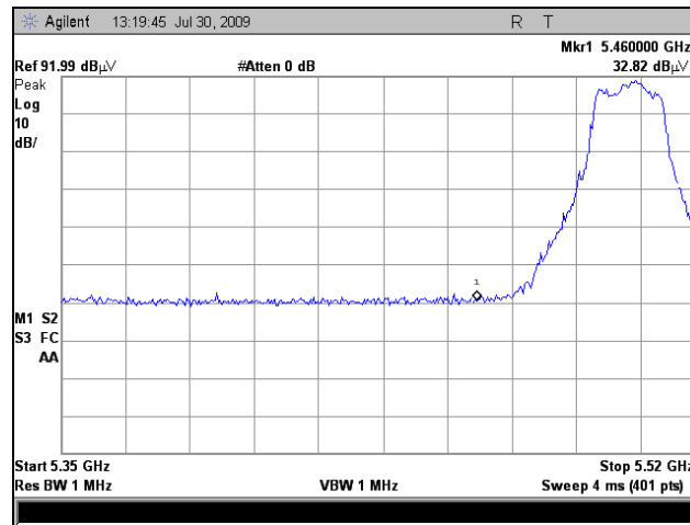
Plot 226. Restricted Band, 802.11n 20MHz, 5460 Peak, 19 dBi Panel
