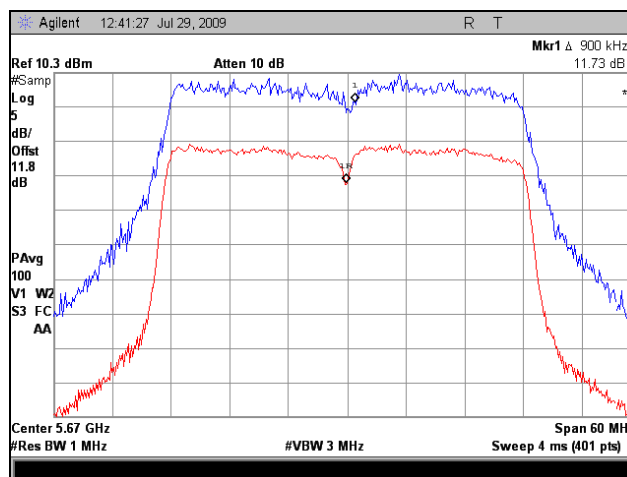
Plot 92. Peak Excursion Ratio, Port 1, 802.11n 40MHz, 5670 MHz
