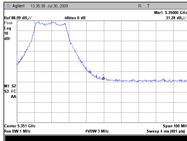
Plot 191. EIRP, 802.11n 20MHz, 5350 MHz Peak, 19 dBi Panel
