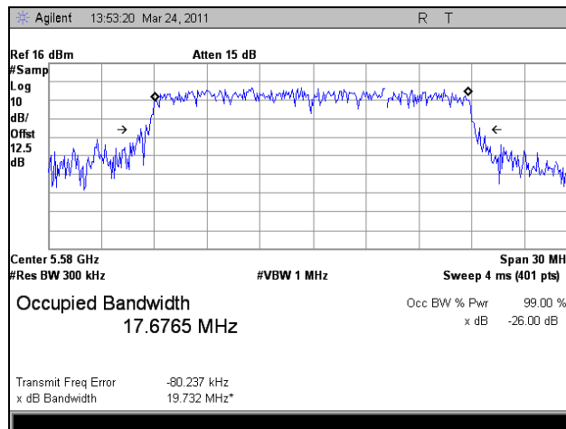
Plot 61. 99% Occupied Bandwidth, Port 2, 802.11n 20MHz, 5580 MHz
