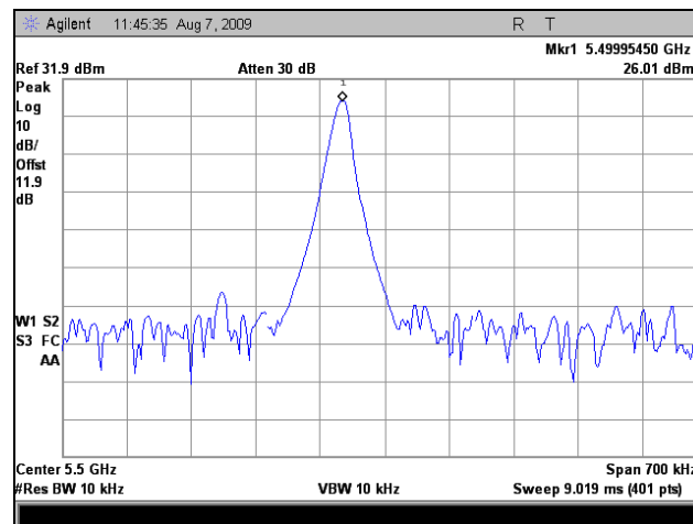
Plot 234. Freq. Stability, Port 1, 5500 MHz @-40C High Volt.
