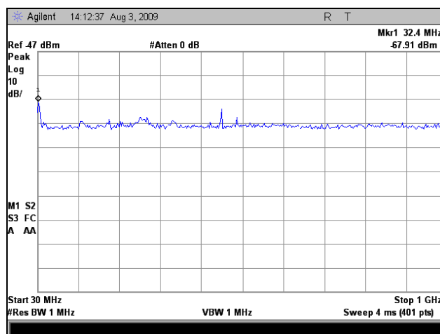
Plot 171. Radiated Spurious, 802.11n 40MHz, 5670 MHz, 30 MHz – 1 GHz, 19 dBi Panel
