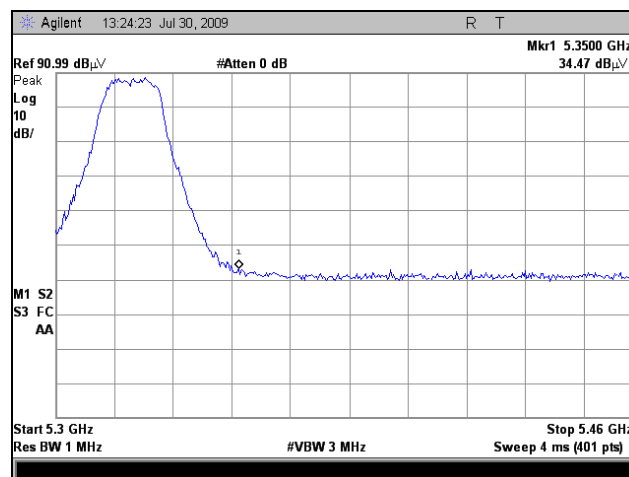
Plot 224. Restricted Band, 802.11n 20MHz, 5350 Peak, 19 dBi Panel
