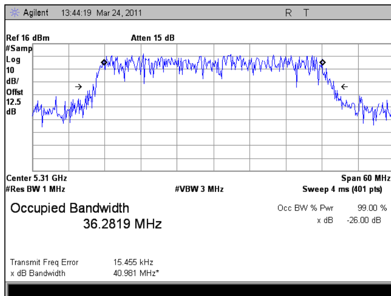
Plot 292. Occupied Bandwidth, 802.11n 40MHz, 5310 MHz
