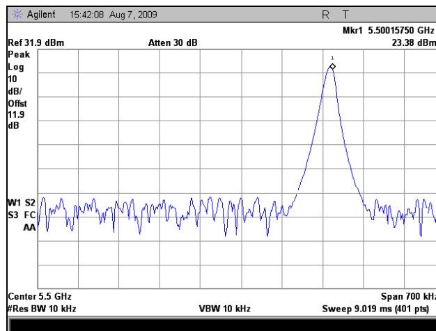
Plot 239. Freq. Stability, Port 1, 5500 MHz @+60C Low Volt.
