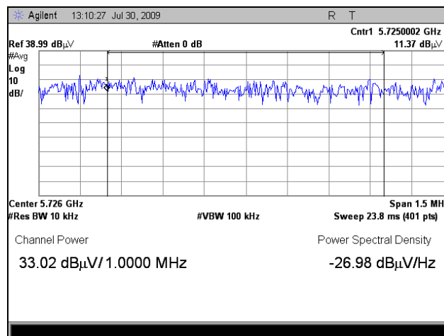
Plot 190. EIRP, Port 1, 802.11a, 5725 MHz Over 1 MHz, 19 dBi Panel
