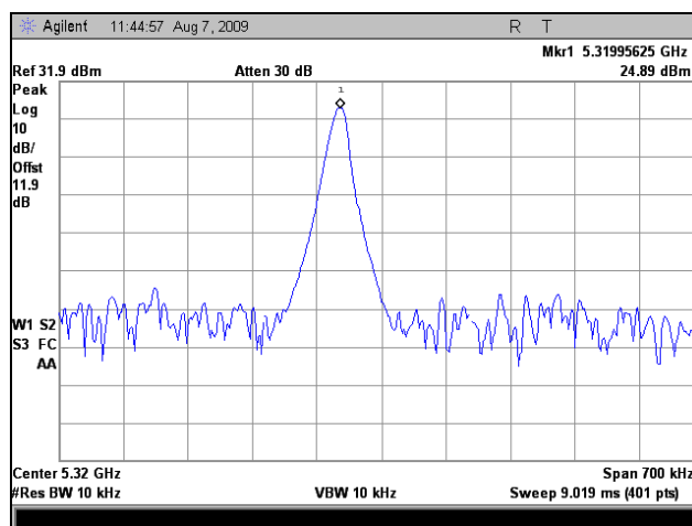
Plot 232. Freq. Stability, Port 1, 5320 MHz @-40C High Volt.
