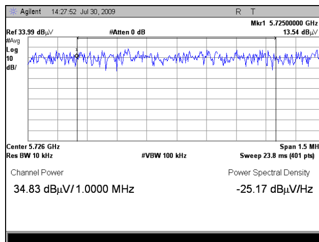
Plot 202. EIRP, 802.11n 40MHz, 5725 MHz Over 1 MHz, 19 dBi Panel
