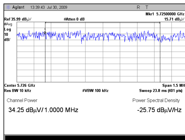
Plot 196. EIRP, 802.11n 20MHz, 5725 MHz Over 1 MHz, 19 dBi Panel
