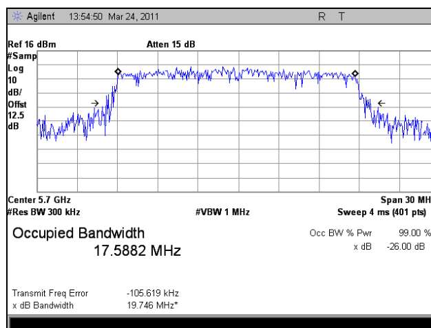
Plot 62. 99% Occupied Bandwidth, Port 2, 802.11n 20MHz, 5700 MHz
