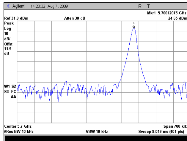
Plot 265. Freq. Stability, Port 3, 5700 MHz @+60C Low Volt.
