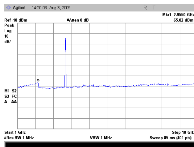
Plot 168. Radiated Spurious, 802.11n 40MHz, 5510 MHz, 1 GHz – 18 GHz, 19 dBi Panel
