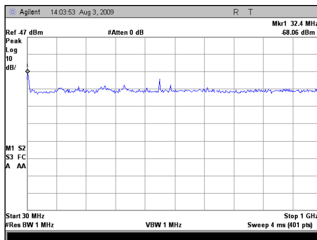
Plot 149. Radiated Spurious, 802.11a, 5580 MHz, 30 MHz – 1 GHz, 19 dBi Panel
