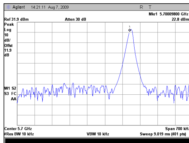
Plot 266. Freq. Stability, Port 3, 5700 MHz @+60C High Volt.
