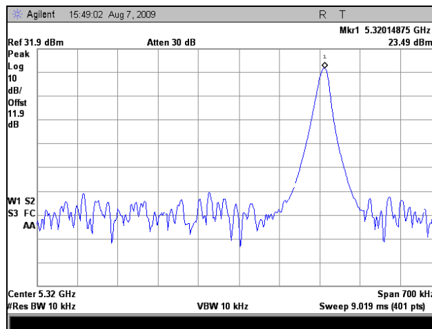
Plot 238. Freq. Stability, Port 1, 5320 MHz @+60C High Volt.
