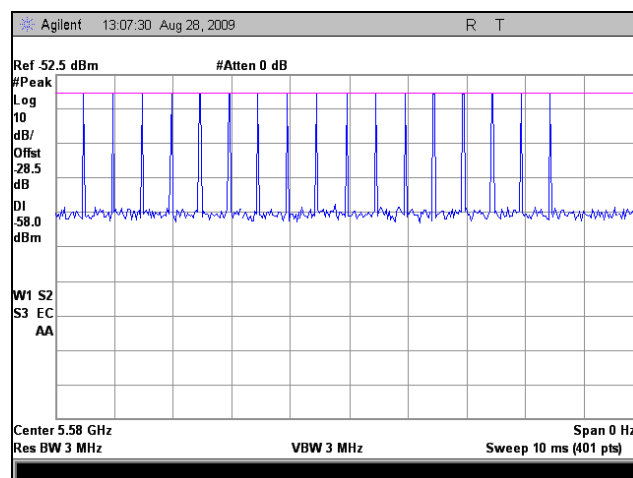
Plot 287. Calibration Plot, Bin 3, 5580 MHz (used for CACT, Bandwidth, Non Occupancy, Close Time & Move Time)
