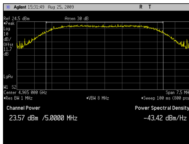
Plot 2. RF Power Output, Low Channel, 802.11a, Mid Channel, 5 MHz
