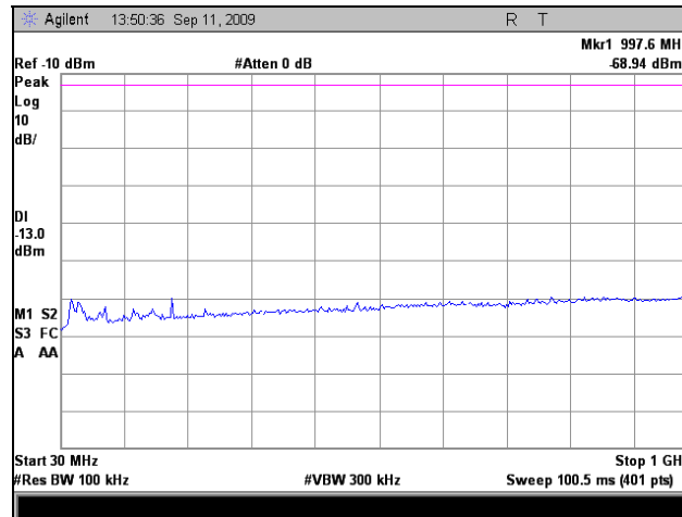
Plot 57. Radiated Spurious Emissions, Low Channel, 5 MHz (30 MHz – 1 GHz)
