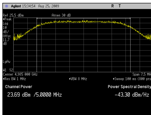
Plot 3. RF Power Output, Low Channel, 802.11a, High Channel, 5 MHz
