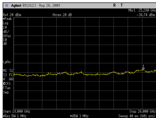
Plot 49. Conducted Spurious Emissions, High Channel, 10 MHz (18 GHz - 26 GHz)
