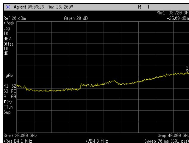
Plot 38. Conducted Spurious Emissions, Mid Channel, 5 MHz (26 GHz – 40 GHz)
