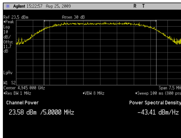
Plot 1. RF Power Output, Low Channel, 802.11a, Low Channel, 5 MHz
