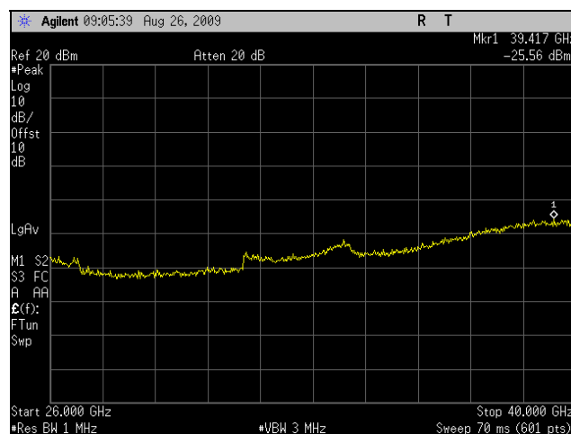
Plot 35. Conducted Spurious Emissions, Low Channel, 5 MHz (26 GHz – 40 GHz)
