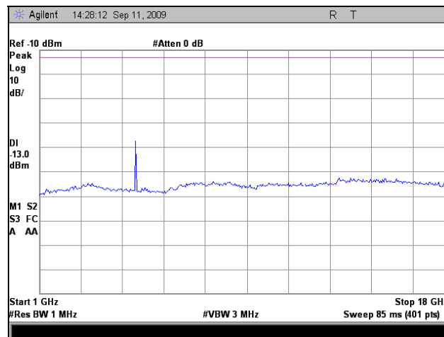
Plot 58. Radiated Spurious Emissions, Low Channel, 5 MHz (1 GHz – 18 GHz)
