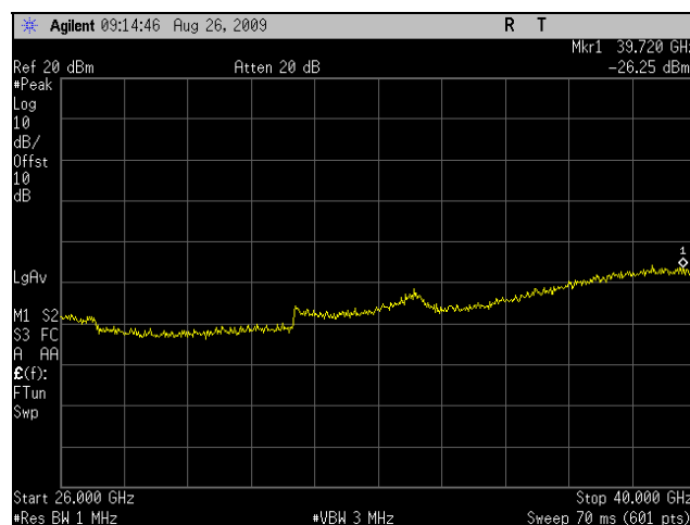
Plot 41. Conducted Spurious Emissions, High Channel, 5 MHz (26 GHz – 40 GHz)
