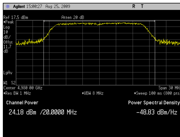
Plot 8. RF Power Output, High Channel, 802.11a, High Channel, 20 MHz
