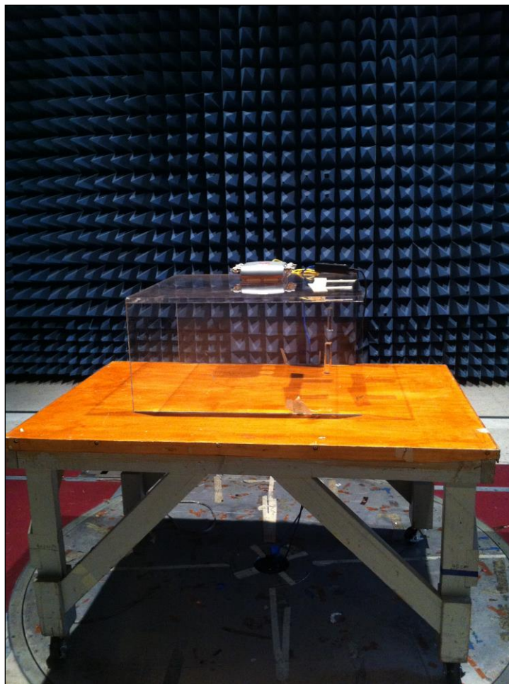
Photograph 1. Radiated Emission Spurious, Test Setup
