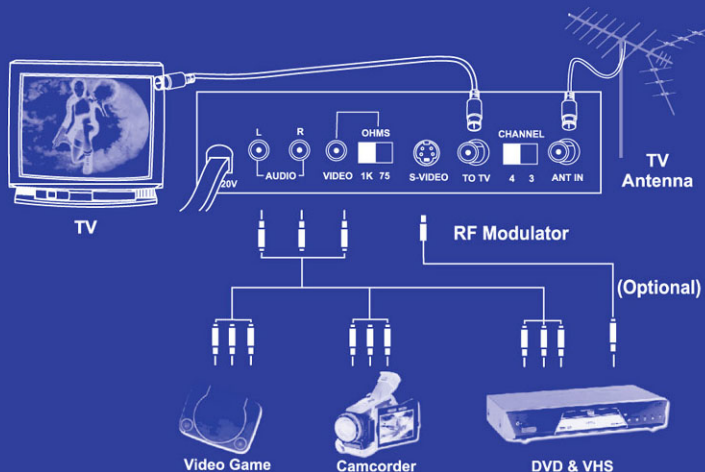
RF Modulator Connection Diagram
