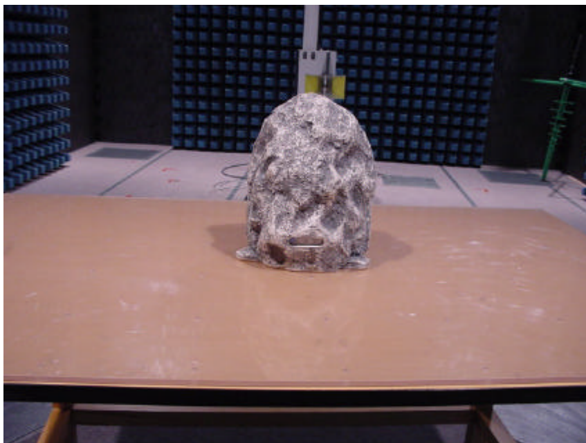
Photograph 3: Set-up for Radiation Measurement Above 1GHz
