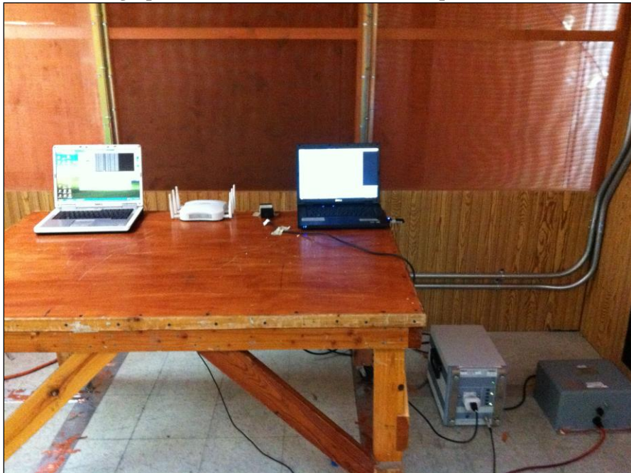
Photograph 8. Conducted Emissions, 15.207(a), Test Setup, AC-DC Power Supply
