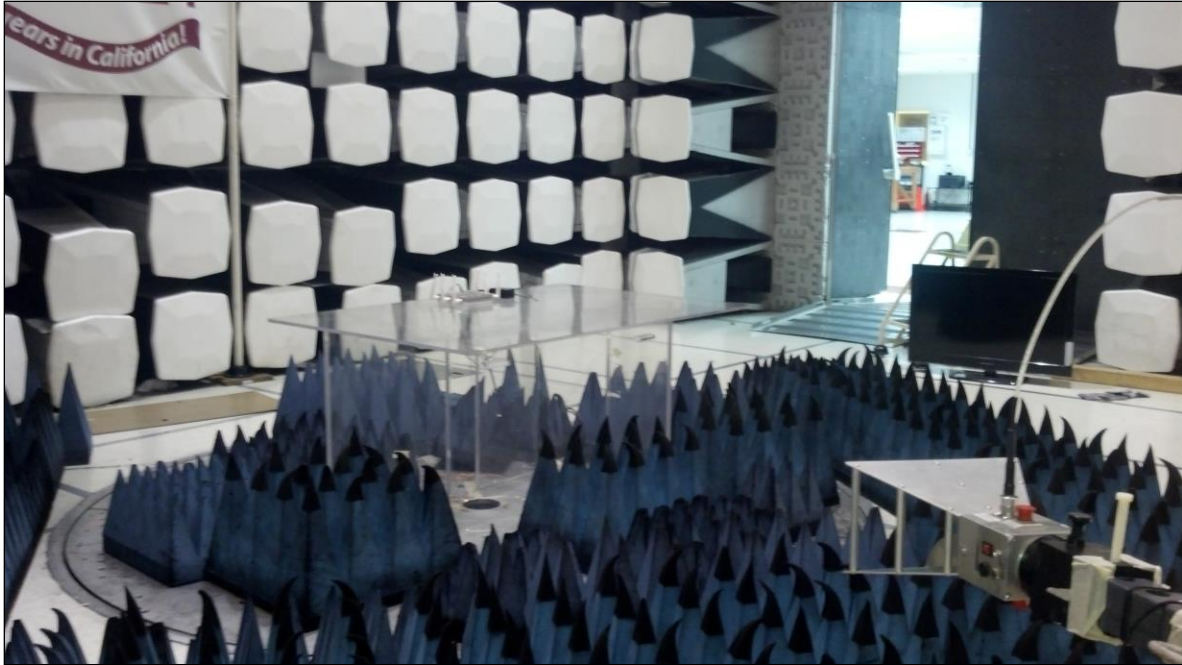
Photograph 7. Radiated Emissions, Test Setup, Above 1 GHz
