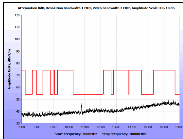
Plot 422. Radiated Spurious Emissions, 802.11n 20 MHz, Mid Channel, 7 GHz – 18 GHz, Omni, 5580 MHz
