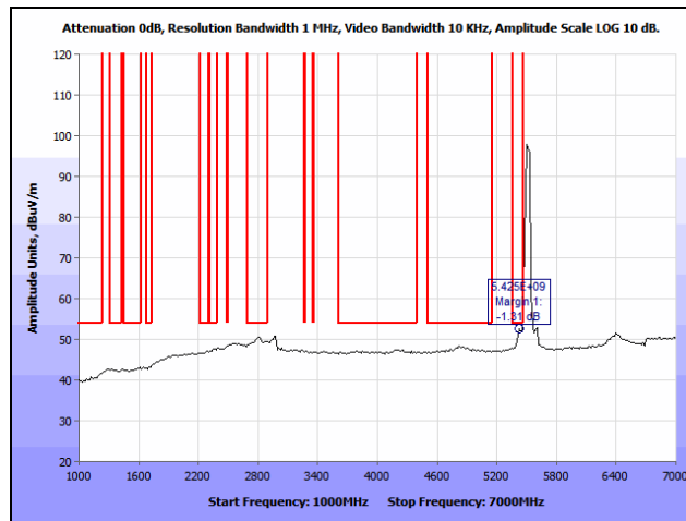
Plot 384. Radiated Spurious Emissions, 802.11n 40 MHz, Low Channel, 1 GHz – 7 GHz, Average, Ceiling, 5510 MHz
