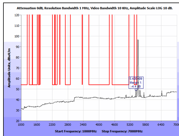
Plot 328. Radiated Spurious Emissions, 802.11n 20 MHz, Low Channel, 1 GHz – 7 GHz, Avg., Patch, 5500 MHz
