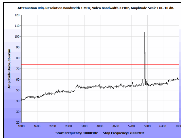
Plot 325. Radiated Spurious Emissions, 802.11a, High Channel, 1 GHz – 7 GHz, Peak, Patch, 5700 MHz
