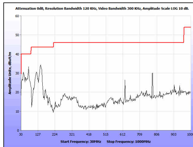
Plot 343. Radiated Spurious Emissions, 802.11n 40 MHz, Mid Channel, 30 MHz – 1 GHz, Patch, 5550 MHz
