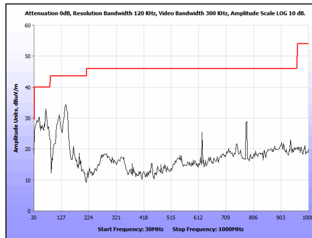
Plot 327. Radiated Spurious Emissions, 802.11n 20 MHz, Low Channel, 30 MHz – 1 GHz, Patch, 5500 MHz
