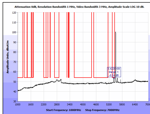
Plot 416. Radiated Spurious Emissions, 802.11n 20 MHz, Low Channel, 1 GHz – 7 GHz, Avg., Omni, 5500 MHz
