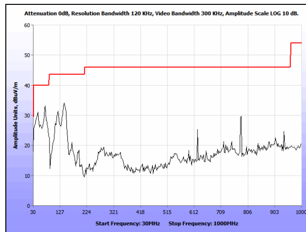
Plot 223. Radiated Spurious Emissions, 802.11n 20 MHz, Mid Channel, 30 MHz – 1 GHz, Patch, 5300 MHz
