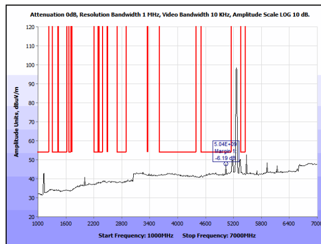
Plot 220. Radiated Spurious Emissions, 802.11n 20 MHz, Low Channel, 1 GHz – 7 GHz, Avg., Patch, 5260 MHz
