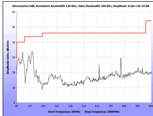
Plot 339. Radiated Spurious Emissions, 802.11n 40 MHz, Low Channel, 30 MHz – 1 GHz, Patch, 5510 MHz
