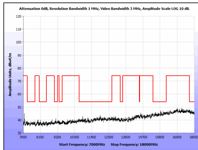
Plot 286. Radiated Spurious Emissions, 802.11a, Mid Channel, 7 GHz – 18 GHz, Omni, 5300 MHz
