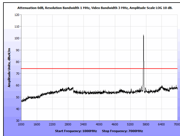
Plot 413. Radiated Spurious Emissions, 802.11a, High Channel, 1 GHz – 7 GHz, Peak, Omni, 5700 MHz
