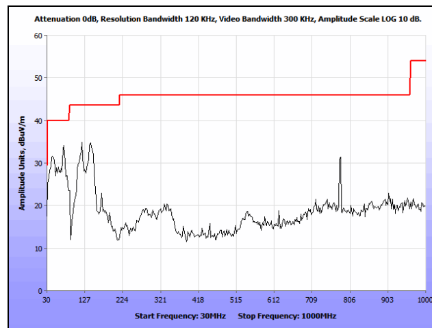
Plot 419. Radiated Spurious Emissions, 802.11n 20 MHz, Mid Channel, 30 MHz – 1 GHz, Omni, 5580 MHz
