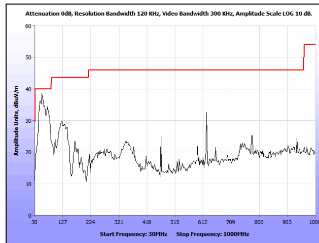
Plot 267. Radiated Spurious Emissions, 802.11n 40 MHz, Low Channel, 30 MHz – 1 GHz, Ceiling, 5270 MHz
