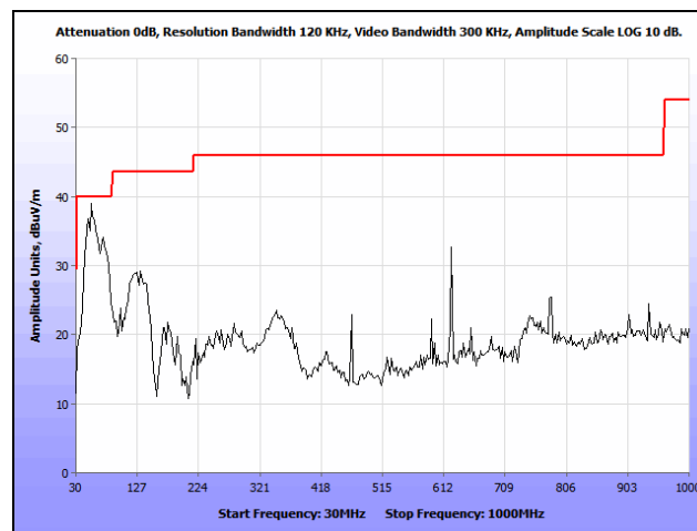
Plot 375. Radiated Spurious Emissions, 802.11n 20 MHz, Mid Channel, 30 MHz – 1 GHz, Ceiling, 5580 MHz
