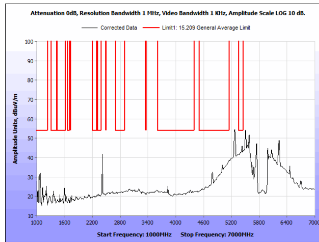
Plot 62. Radiated Spurious Emissions, 802.11n 20 MHz, High Channel, 1 GHz – 7 GHz, Average
