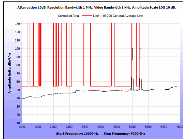
Plot 170. Radiated Spurs, Co-Location, 802.11n 20 MHz, 5200 MHz & 5580 MHz, 1 GHz – 7 GHz, Avg., Omni
