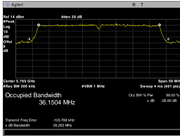
Plot 26. 26 dB Occupied Bandwidth, 802.11n, 5795 MHz, Port 2
