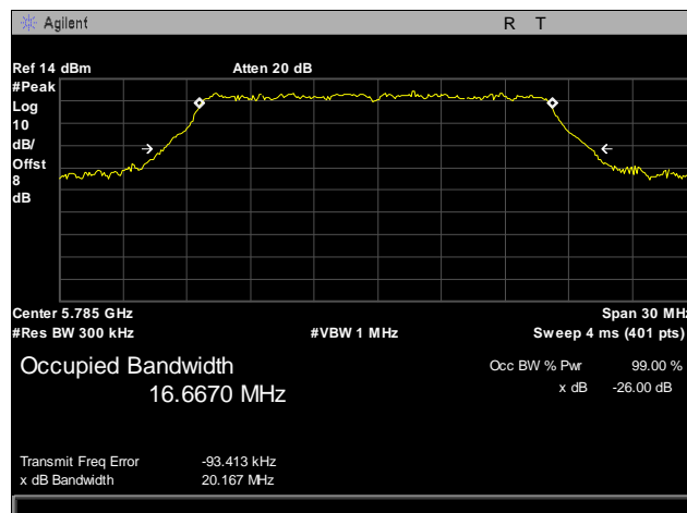
Plot 15. 26 dB Occupied Bandwidth, 802.11a, 5785 MHz
