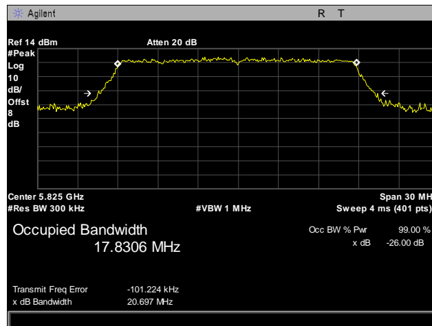
Plot 27. 26 dB Occupied Bandwidth, 802.11n, 5825 MHz, Port 2
