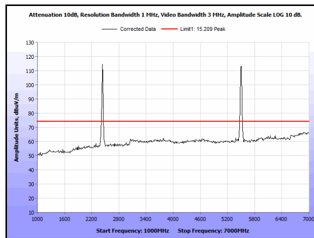
Plot 227. Radiated Spurs, Co-Location, 802.11n 20 MHz, 2437 MHz & 5580 MHz, 1 GHz – 7 GHz, Peak, Patch
