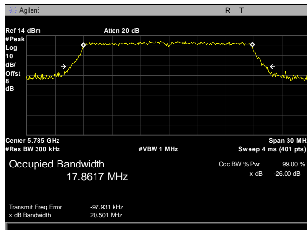
Plot 20. 26 dB Occupied Bandwidth, 802.11n, 5785 MHz, Port 1
