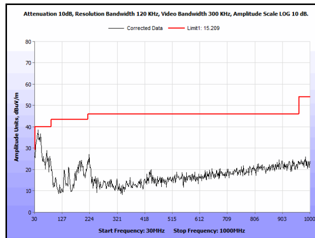
Plot 169. Radiated Spurs, Co-Location, 802.11n 20 MHz, 5200 MHz & 5580 MHz, 30 MHz – 1 GHz, Peak, Omni
