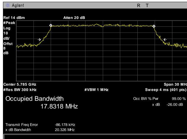
Plot 25. 26 dB Occupied Bandwidth, 802.11n, 5785 MHz, Port 2
