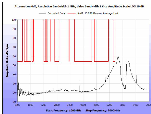
Plot 70. Radiated Spurious Emissions, 802.11ac 80 MHz, 1 GHz – 7 GHz, Average
