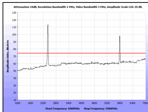
Plot 215. Radiated Spurs, Co-Location, 802.11n 20 MHz, 2412 MHz & 5785 MHz, 1 GHz – 7 GHz, Peak, Patch
