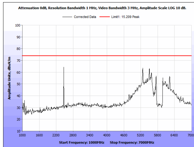
Plot 40. Radiated Spurious Emissions, 802.11a 20 MHz, Mid Channel, 1 GHz – 7 GHz, Peak
