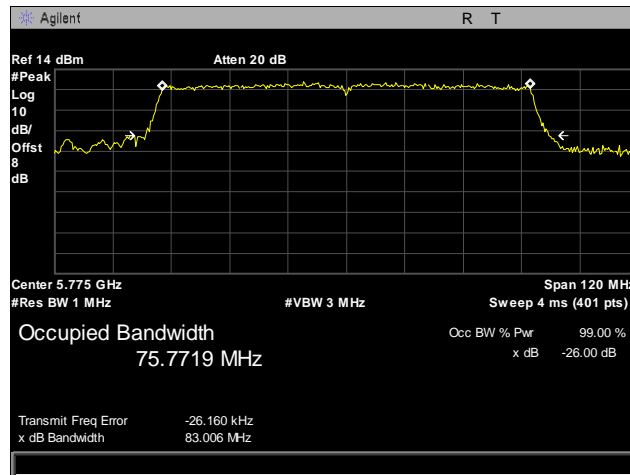
Plot 28. 26 dB Occupied Bandwidth, 802.11ac, 5775 MHz, Port 1
