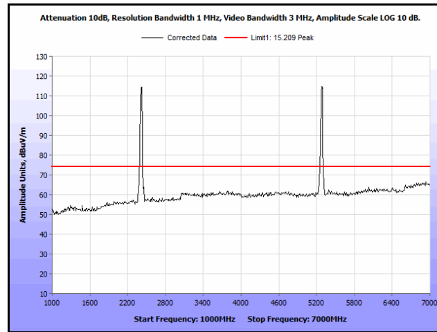
Plot 207. Radiated Spurs, Co-Location, 802.11n 20 MHz, 2412 MHz & 5300 MHz, 1 GHz – 7 GHz, Peak, Patch
