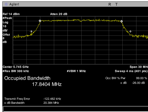
Plot 23. 26 dB Occupied Bandwidth, 802.11n, 5745 MHz, Port 2
