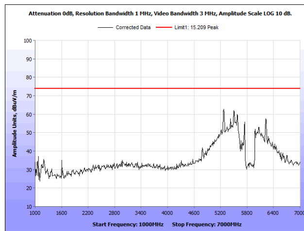
Plot 63. Radiated Spurious Emissions, 802.11n 20 MHz, High Channel, 1 GHz – 7 GHz, Peak
