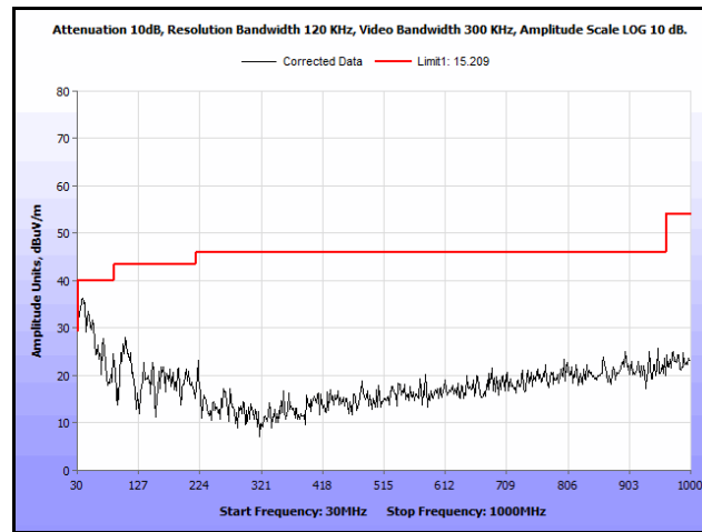
Plot 161. Radiated Spurs, Co-Location, 802.11n 20 MHz, 5200 MHz & 5200 MHz, 30 MHz – 1 GHz, Peak, Omni
