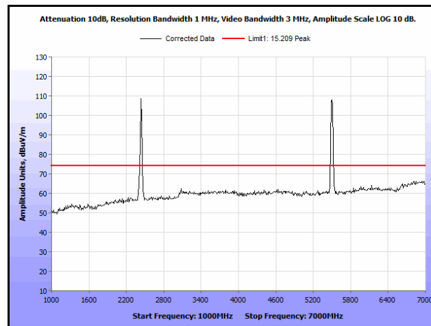
Plot 139. Radiated Spurs, Co-Location, 802.11n 20 MHz, 2437 MHz & 5580 MHz, 1 GHz – 7 GHz, Peak, Omni
