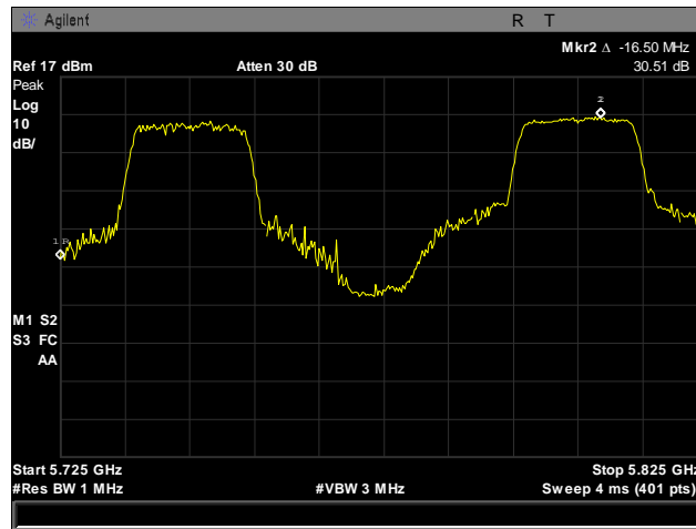
Plot 249. Frequency Stability, 5725 – 5825 MHz, -40°C, 120 V
