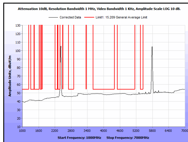
Plot 230. Radiated Spurs, Co-Location, 802.11n 20 MHz, 2437 MHz & 5785 MHz, 1 GHz – 7 GHz, Avg., Patch
