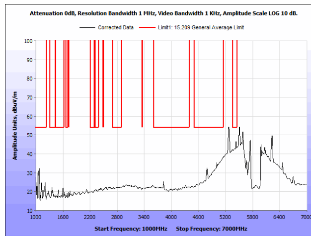
Plot 50. Radiated Spurious Emissions, 802.11n 20 MHz, Low Channel, 1 GHz – 7 GHz, Average
