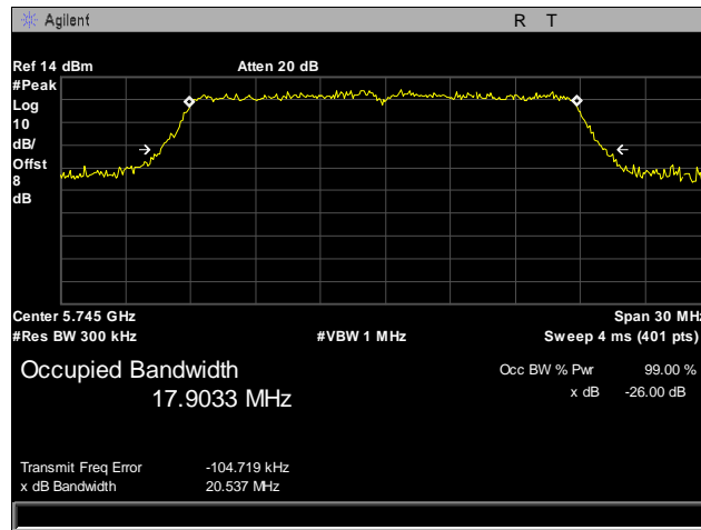
Plot 18. 26 dB Occupied Bandwidth, 802.11n, 5745 MHz, Port 1
