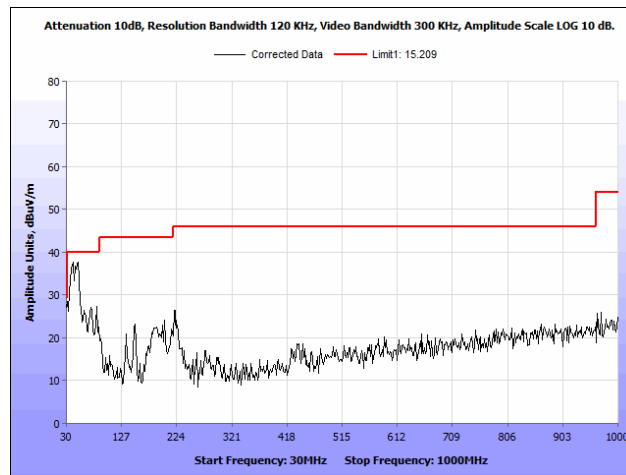
Plot 65. Radiated Spurious Emissions, 802.11n 40 MHz, High Channel, 30 MHz – 1 GHz
