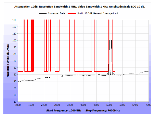
Plot 166. Radiated Spurs, Co-Location, 802.11n 20 MHz, 5200 MHz & 5300 MHz, 1 GHz – 7 GHz, Avg., Omni
