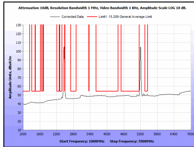
Plot 234. Radiated Spurs, Co-Location, 802.11n 20 MHz, 2462 MHz & 5200 MHz, 1 GHz – 7 GHz, Avg., Patch
