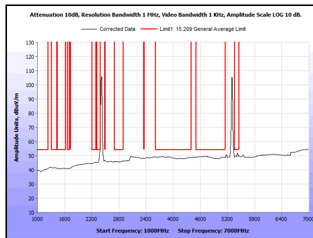
Plot 206. Radiated Spurs, Co-Location, 802.11n 20 MHz, 2412 MHz & 5300 MHz, 1 GHz – 7 GHz, Avg., Patch
