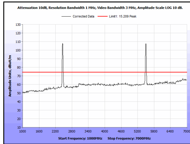
Plot 155. Radiated Spurs, Co-Location, 802.11n 20 MHz, 2462 MHz & 5580 MHz, 1 GHz – 7 GHz, Peak, Omni
