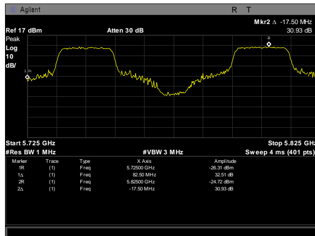
Plot 251. Frequency Stability, 5725 – 5825 MHz, -20°C, 120 V
