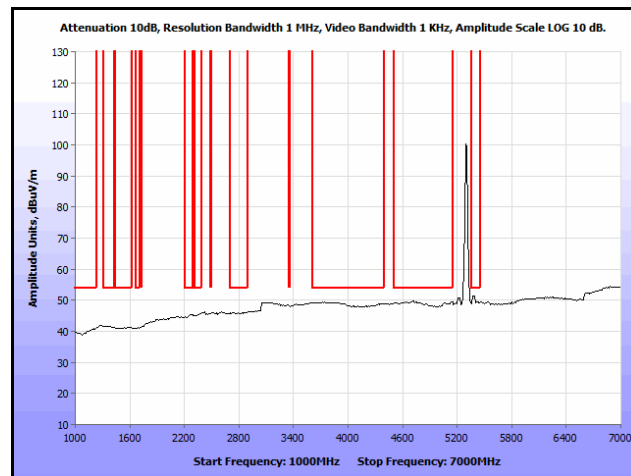
Plot 178. Radiated Spurs, Co-Location, 802.11n 20 MHz, 5300 MHz & 5300 MHz, 1 GHz – 7 GHz, Avg., Omni
