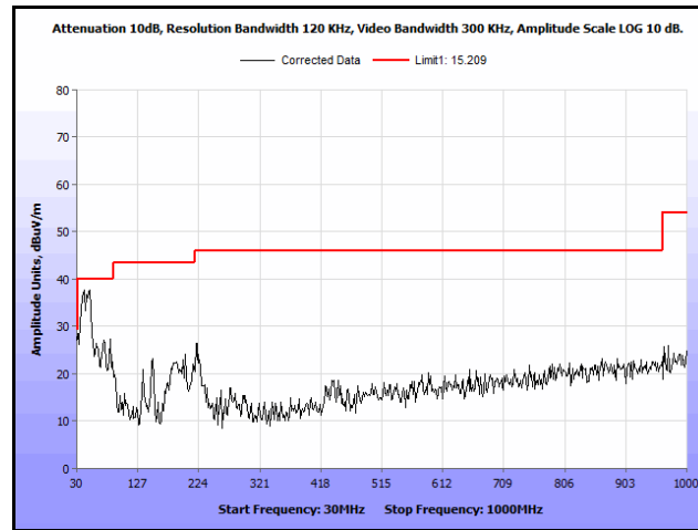
Plot 213. Radiated Spurs, Co-Location, 802.11n 20 MHz, 2412 MHz & 5785 MHz, 30 MHz – 1 GHz, Peak, Patch
