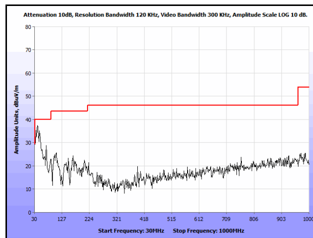
Plot 133. Radiated Spurs, Co-Location, 802.11n 20 MHz, 2437 MHz & 5300 MHz, 30 MHz – 1 GHz, Peak, Omni
