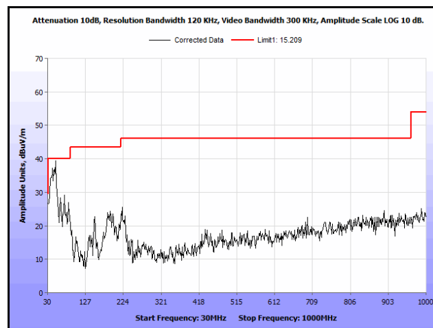
Plot 209. Radiated Spurs, Co-Location, 802.11n 20 MHz, 2412 MHz & 5580 MHz, 30 MHz – 1 GHz, Peak, Patch
