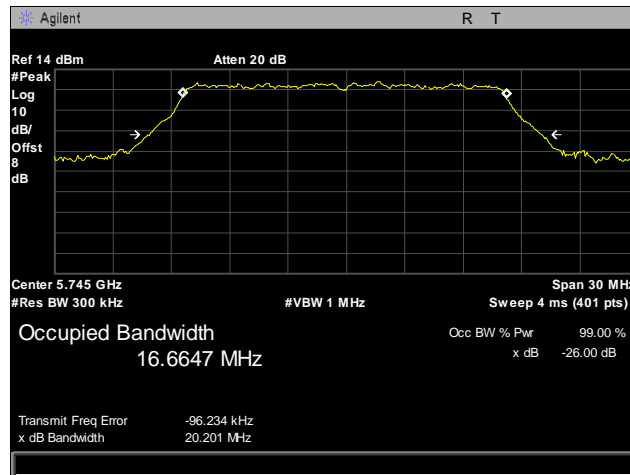
Plot 13. 26 dB Occupied Bandwidth, 802.11a, 5745 MHz
