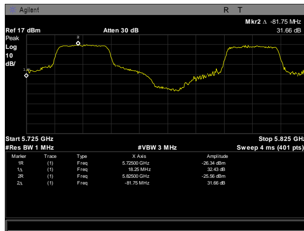
Plot 250. Frequency Stability, 5725 – 5825 MHz, -30°C, 120 V
