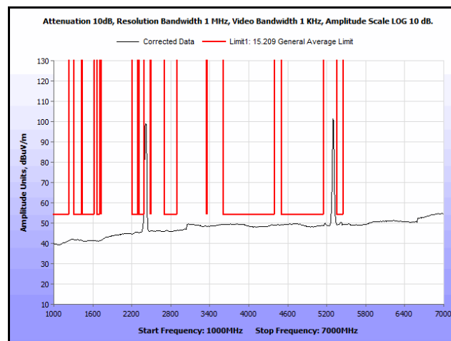
Plot 118. Radiated Spurs, Co-Location, 802.11n 20 MHz, 2412 MHz & 5300 MHz, 1 GHz – 7 GHz, Avg., Omni
