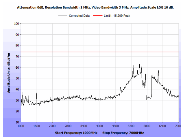
Plot 59. Radiated Spurious Emissions, 802.11n 20 MHz, Mid Channel, 1 GHz – 7 GHz, Peak
