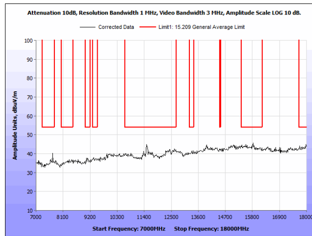
Plot 56. Radiated Spurious Emissions, 802.11n 40 MHz, Low Channel, 7 GHz – 18 GHz
