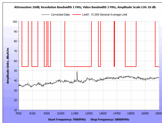
Plot 60. Radiated Spurious Emissions, 802.11n 20 MHz, Mid Channel, 7 GHz – 18 GHz
