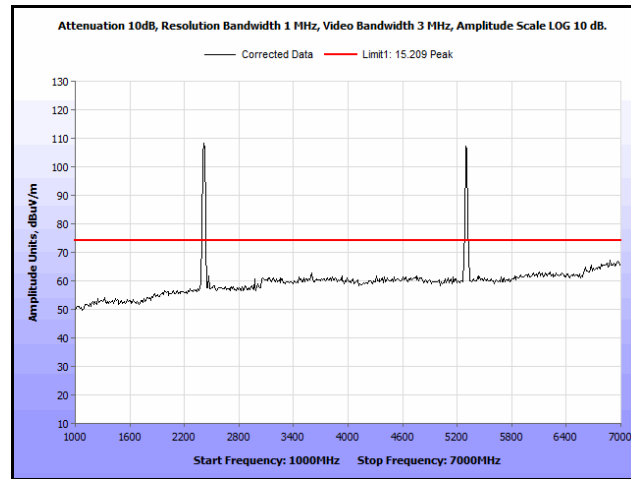
Plot 119. Radiated Spurs, Co-Location, 802.11n 20 MHz, 2412 MHz & 5300 MHz, 1 GHz – 7 GHz, Peak, Omni
