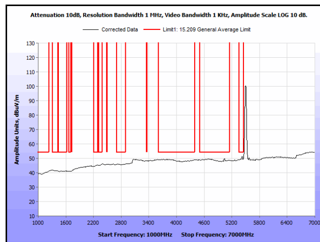
Plot 190. Radiated Spurs, Co-Location, 802.11n 20 MHz, 5580 MHz & 5580 MHz, 1 GHz – 7 GHz, Avg., Omni
