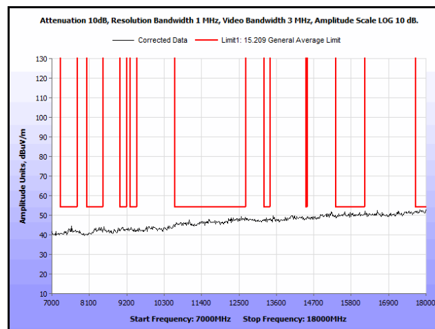
Plot 160. Radiated Spurs, Co-Location, 802.11n 20 MHz, 2462 MHz & 5785 MHz, 7 GHz – 18 GHz, Peak, Omni
