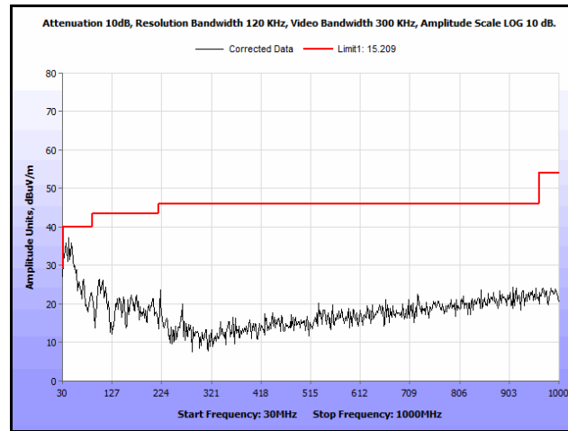
Plot 225. Radiated Spurs, Co-Location, 802.11n 20 MHz, 2437 MHz & 5580 MHz, 30 MHz – 1 GHz, Peak, Patch
