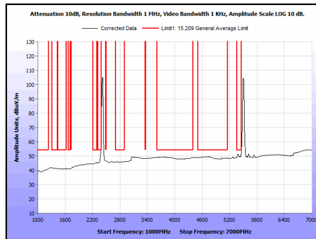
Plot 242. Radiated Spurs, Co-Location, 802.11n 20 MHz, 2462 MHz & 5580 MHz, 1 GHz – 7 GHz, Avg., Patch
