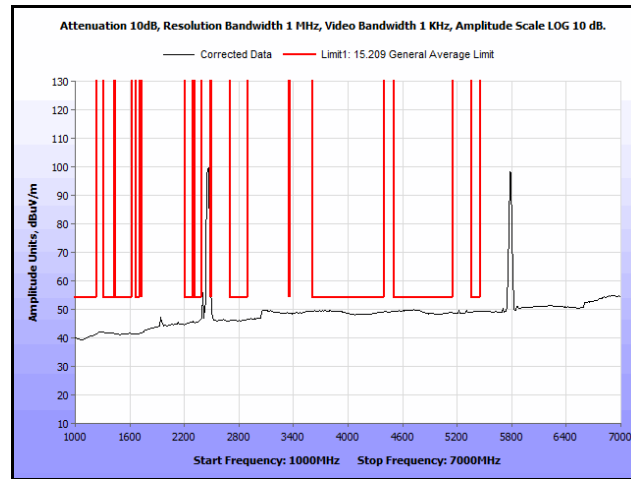
Plot 158. Radiated Spurs, Co-Location, 802.11n 20 MHz, 2462 MHz & 5785 MHz, 1 GHz – 7 GHz, Avg., Omni
