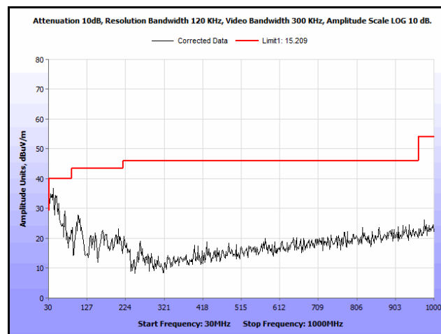
Plot 157. Radiated Spurs, Co-Location, 802.11n 20 MHz, 2462 MHz & 5785 MHz, 30 MHz – 1 GHz, Peak, Omni
