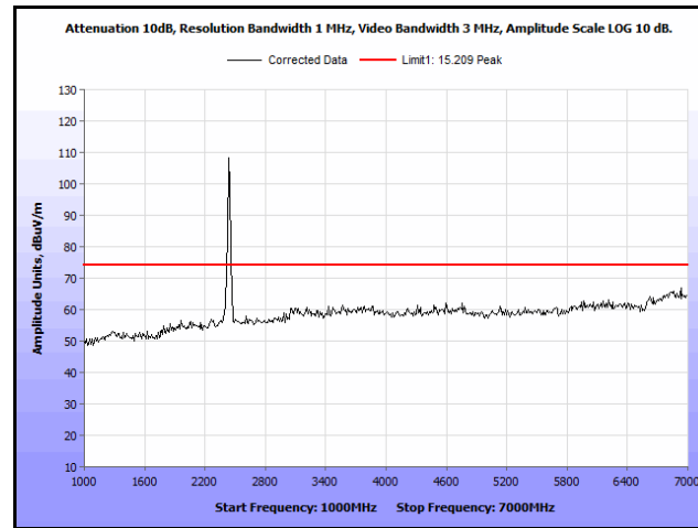
Plot 107. Radiated Spurs, Co-Location, 802.11n 20 MHz, 2437 MHz & 2462 MHz, 1 GHz – 7 GHz, Peak, Omni
