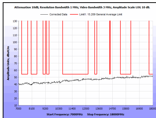
Plot 196. Radiated Spurs, Co-Location, 802.11n 20 MHz, 5580 MHz & 5785 MHz, 7 GHz – 18 GHz, Peak, Omni
