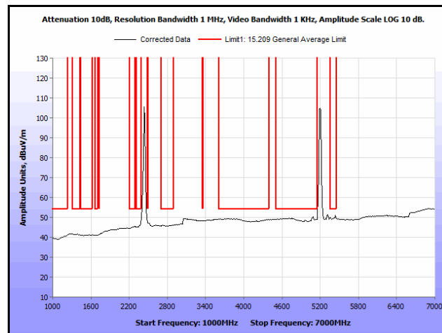
Plot 218. Radiated Spurs, Co-Location, 802.11n 20 MHz, 2437 MHz & 5200 MHz, 1 GHz – 7 GHz, Avg., Patch
