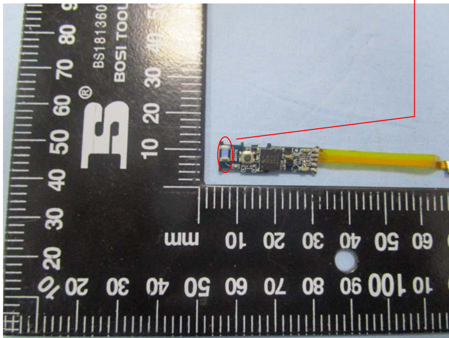
Solder Board-Component View 1 (Bluetooth headset)
