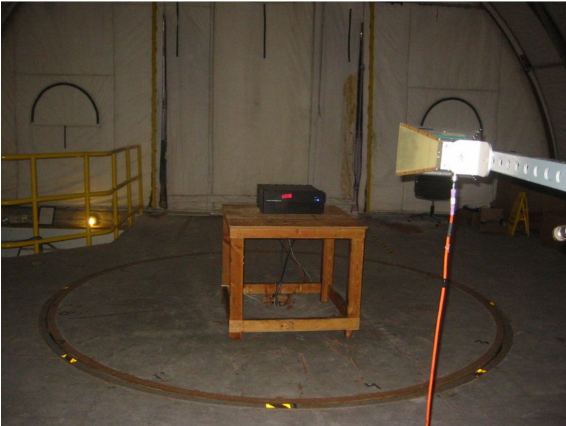
Figure 3: Test Setup Photo 3
