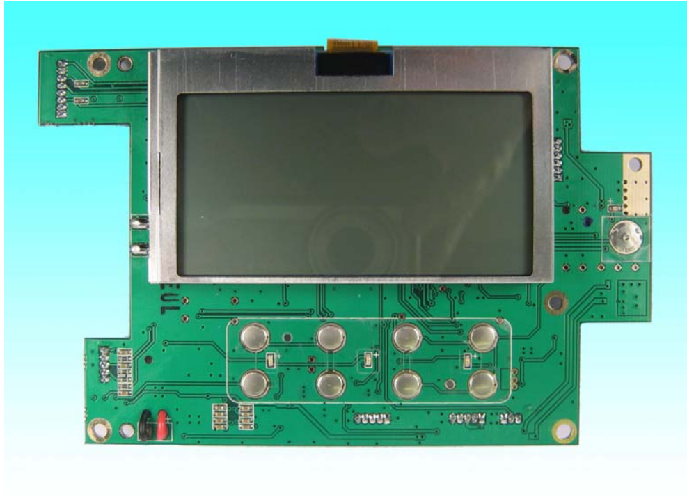
CPU UNIT TOP VIEW – 1
