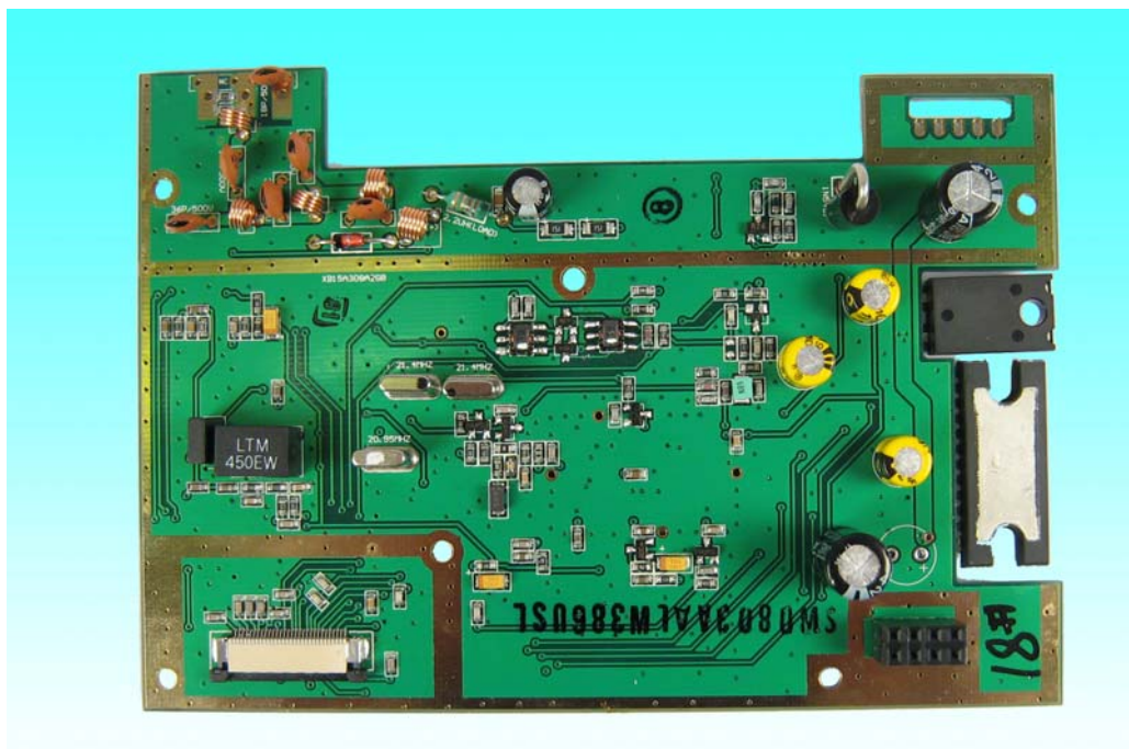
RF UNIT TOP VIEW 1
