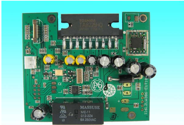
PA HAILER UNIT TOP VIEW
