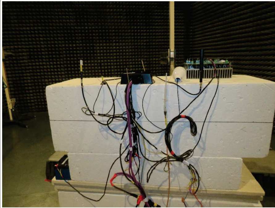
EUT Test setup with antenna
