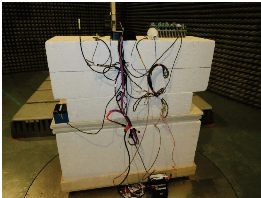
EUT Test setup without antenna
