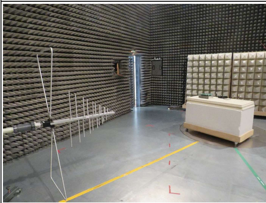
Setup below 1 GHz
