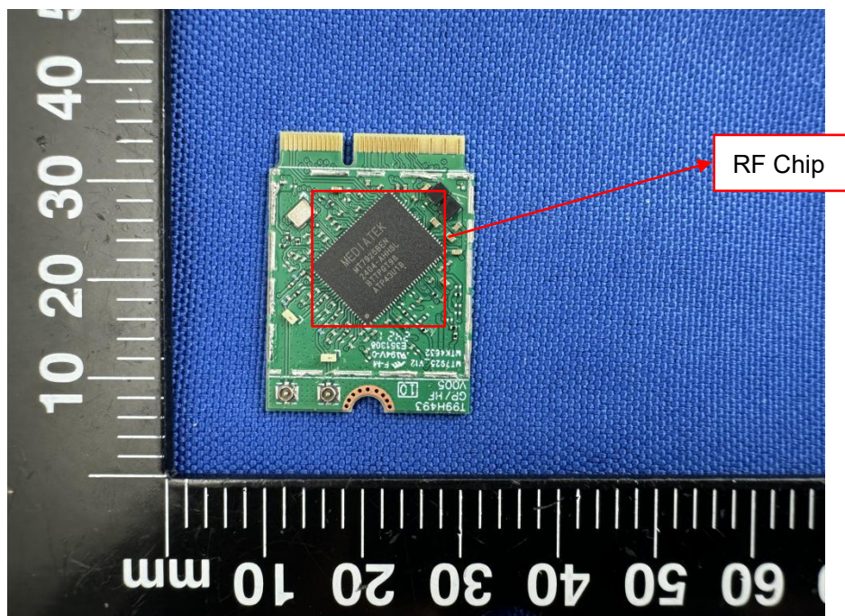
RF MODULE TOP VIEW-MT7925B22M(WITHOUT SHIELDING)
