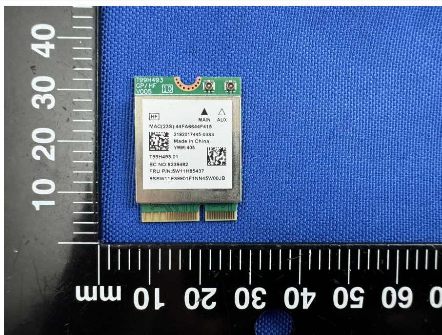
RF MODULE TOP VIEW-MT7925B22M(WITH SHIELDING)
