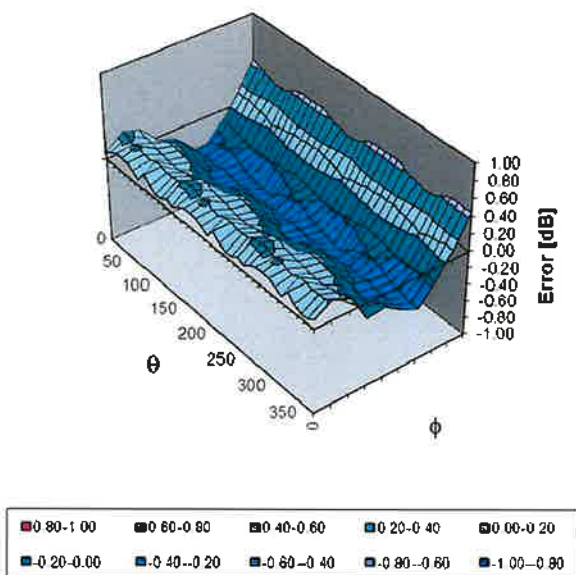
60 GHz: 3D isotropy, E-field parallel to probe axis
