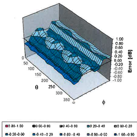
30 GHz: 3D isotropy, E-field parallel to probe axis
