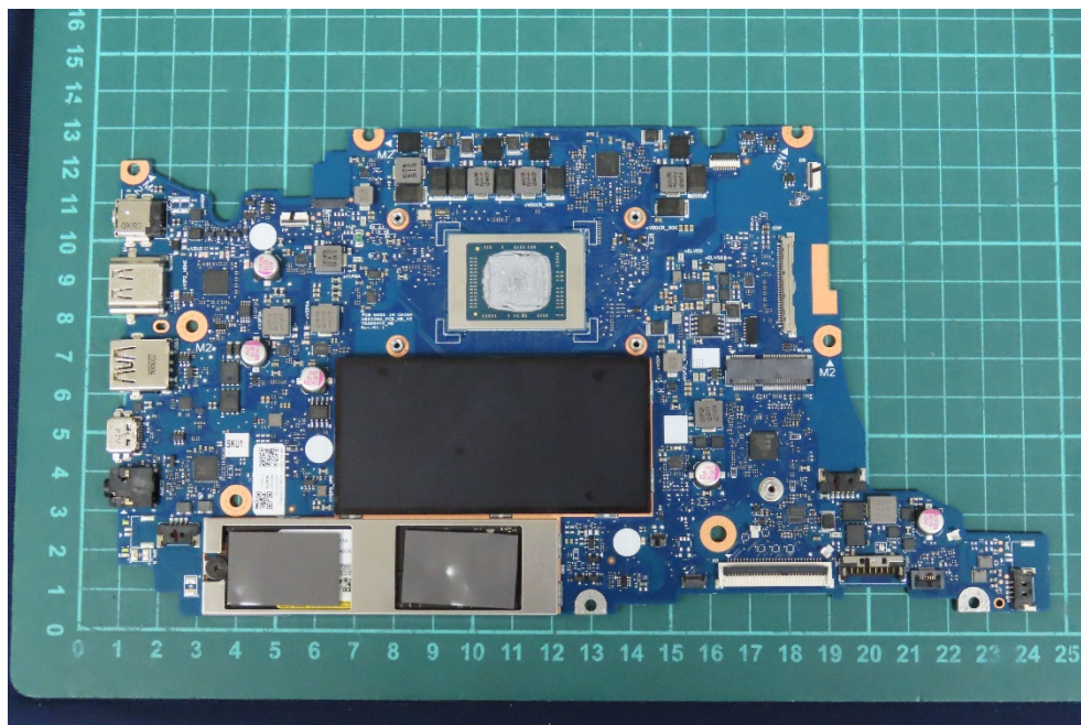
(26) EUT Photo
