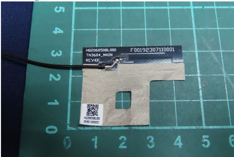
(36) EUT Photo_Antenna: INNOWAVE (Main)
