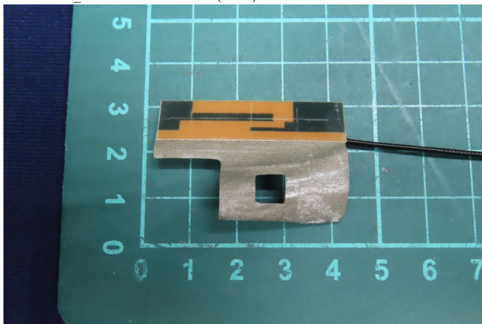
(37) EUT Photo_Antenna: INNOWAVE (Main)
