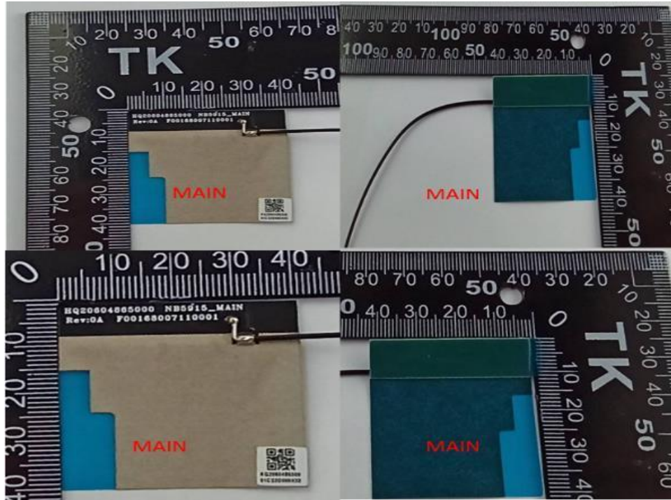
Main Antenna Photo (Front/Back):
