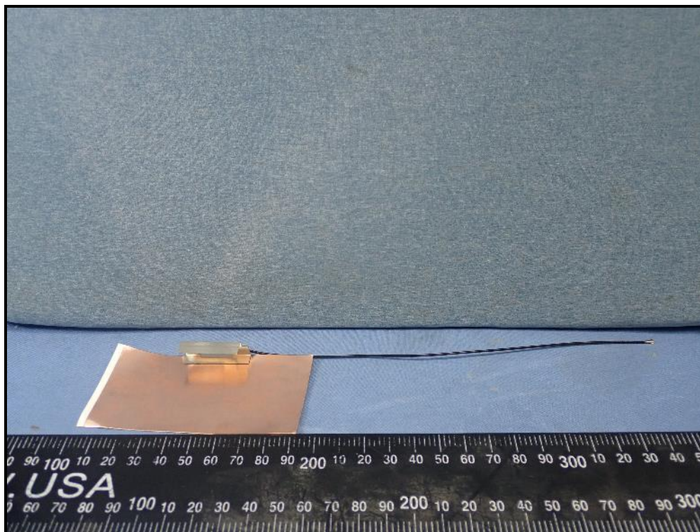
PIFA Antenna (Model: RFMTA311020EMMB301)
