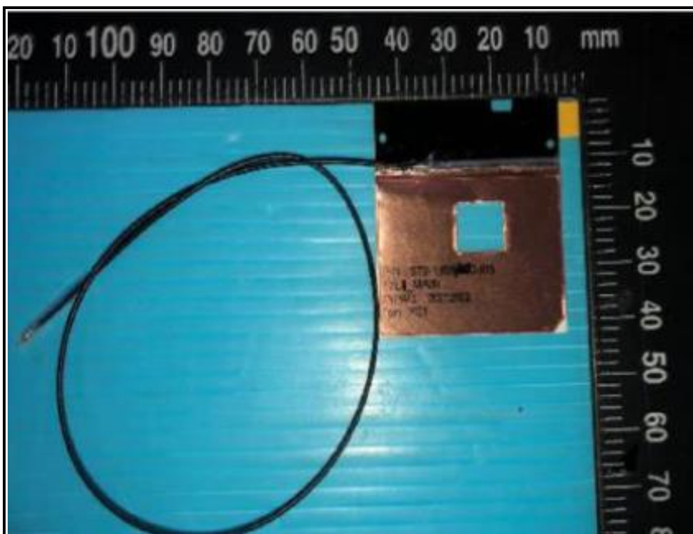
PIFA Antenna (Model: WA-P-LE-02-045 (Main))
