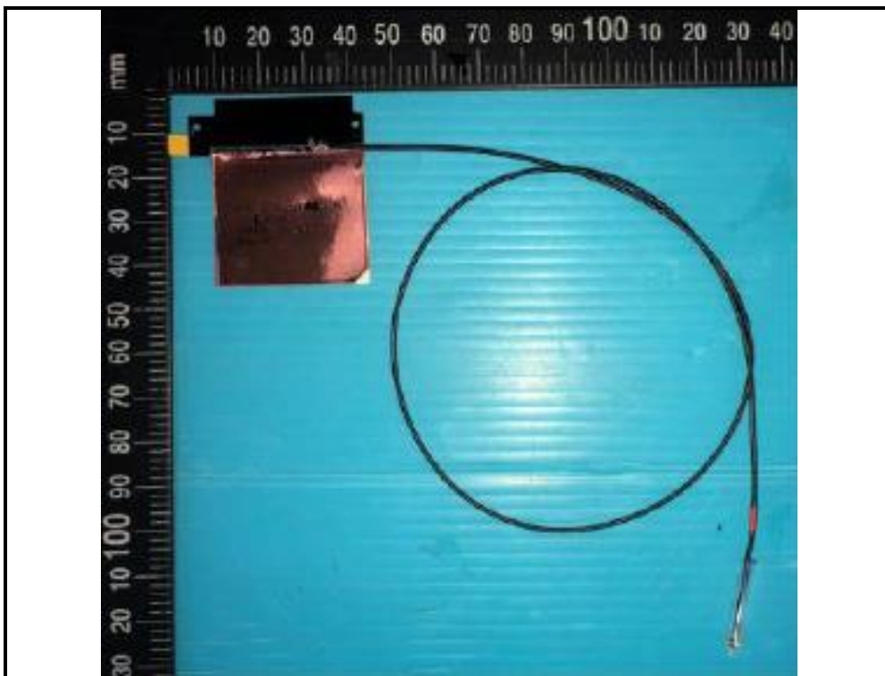
PIFA Antenna (Model: WA-P-LE-02-046 (Aux))
