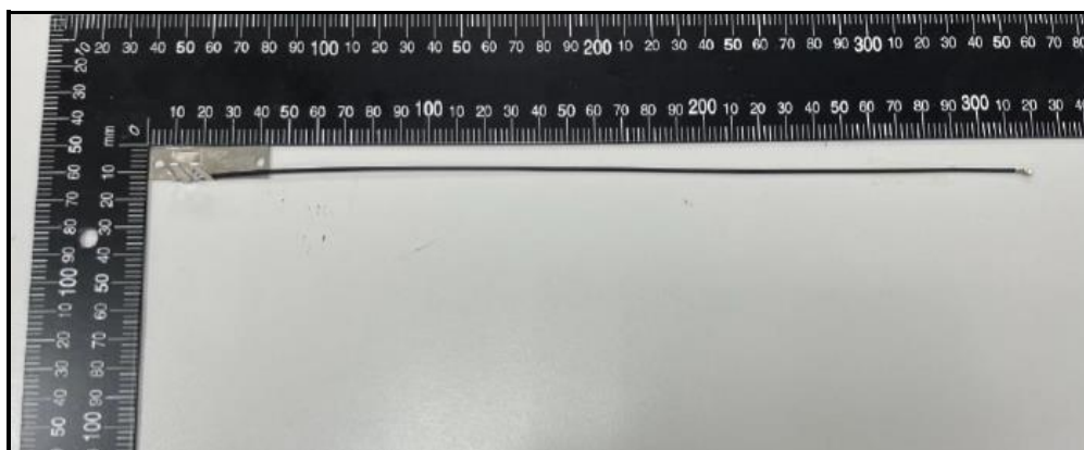
PIFA Antenna (Model: RFMTA421230IMMB701)
