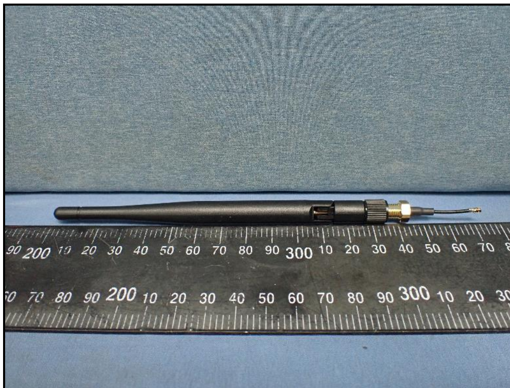
Dipole Antenna (Model: JR2Q00340-1)
