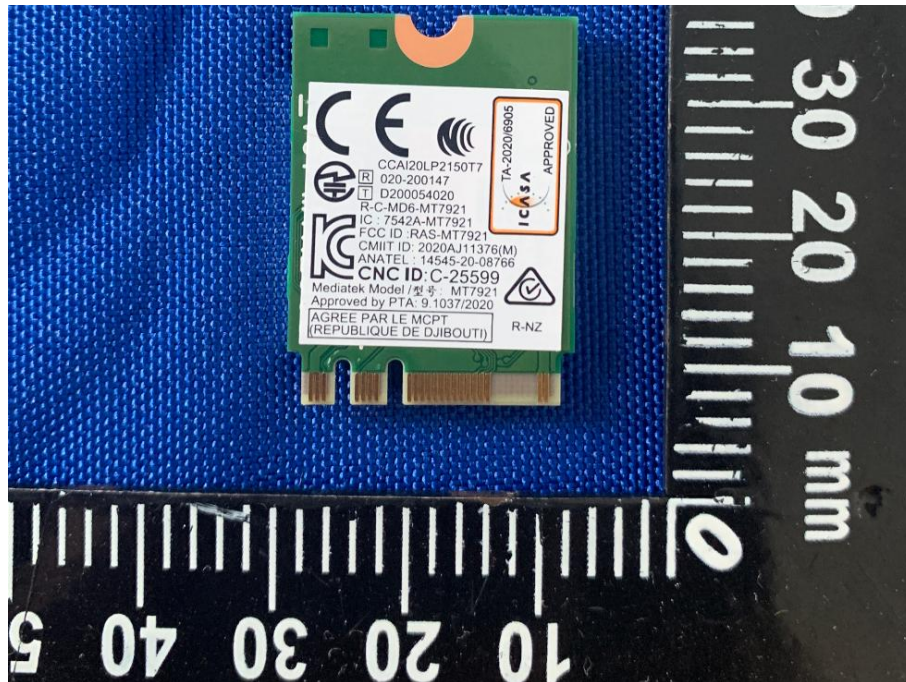
RF MODULE REAR VIEW -MT7921
