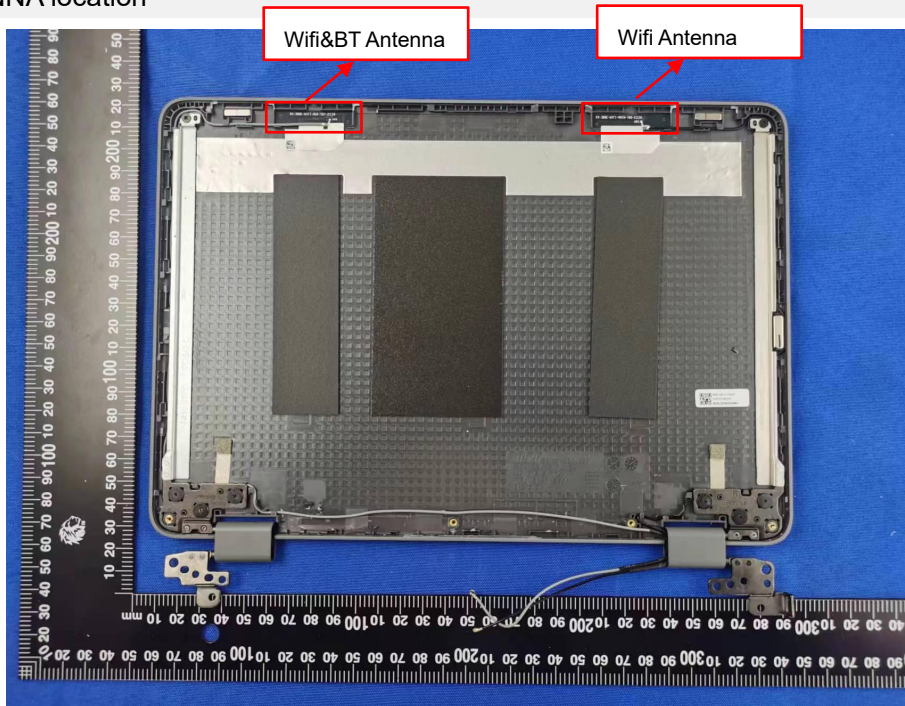
ANTENNA location
