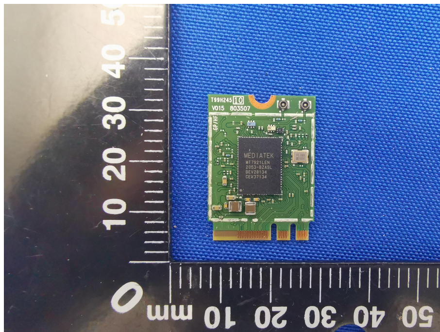
RF MODULE TOP VIEW-MT7921(WITHOUT SHIELDING)
