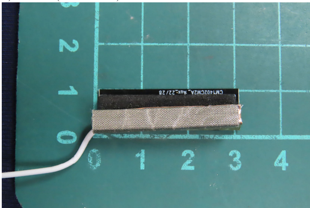
(28) EUT Photo (Antenna-AWAN)
