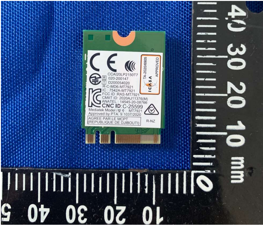
RF MODULE REAR VIEW -MT7921
