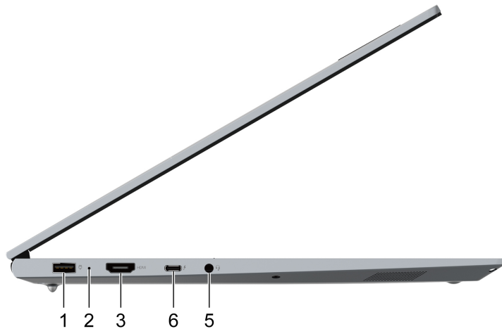
Figure 2. Left view — ThinkBook 16p NX IAP
