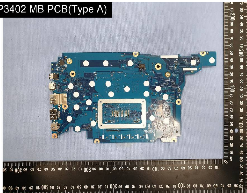
TP3402 MB PCB(Type A)
