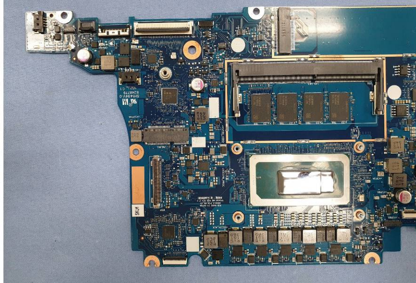
TP3402 MB PCB(Type A)
