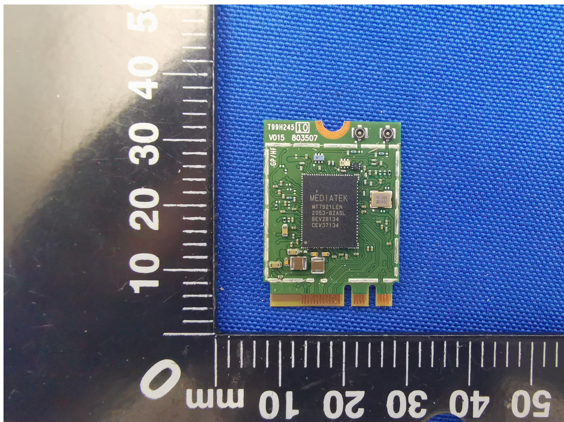
RF MODULE TOP VIE(WITHOUT THE SHIELDING)_MT7921
