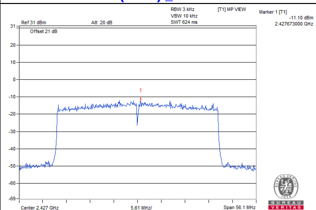
802.11ax (HE20) Chain 0 / CH4
