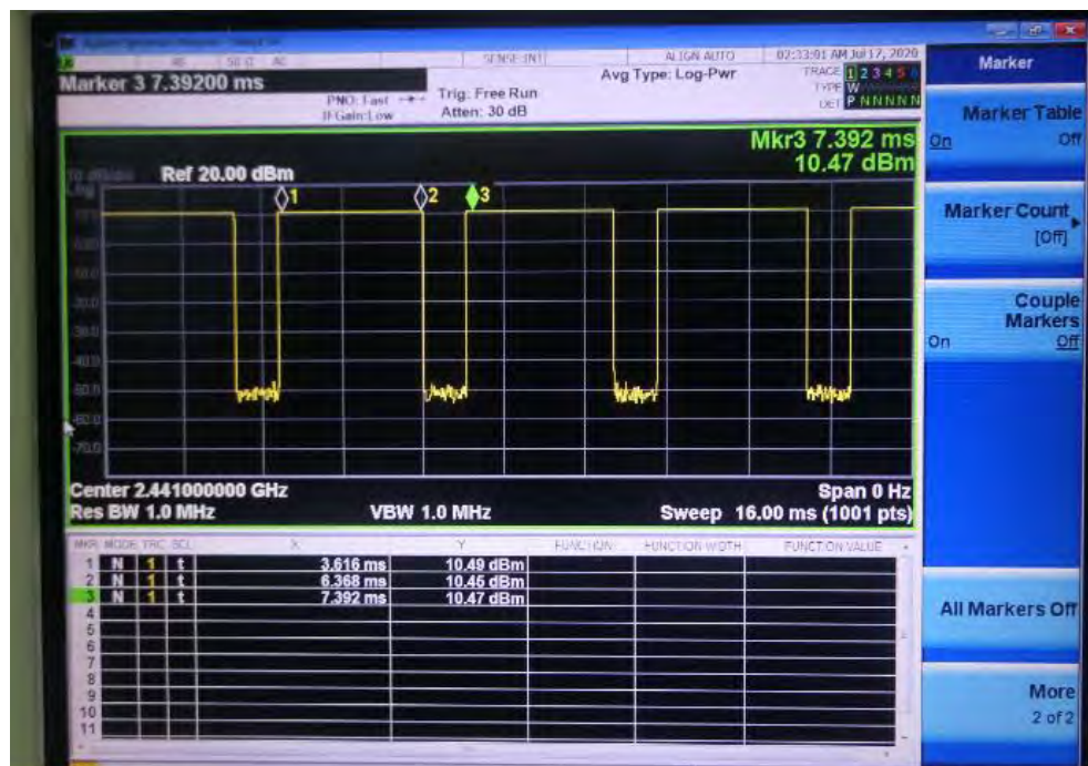
Time-domain plot for Bluetooth transmission signal
