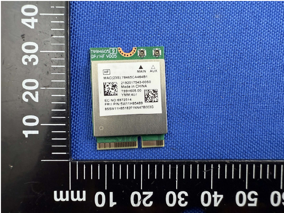
RF MODULE TOP VIEW-MT7920(WITH SHIELDING)
