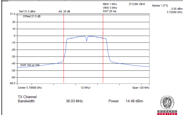
802.11ac (VHT40)_Chain 1 / CH142 (U-NII-2C Band)
