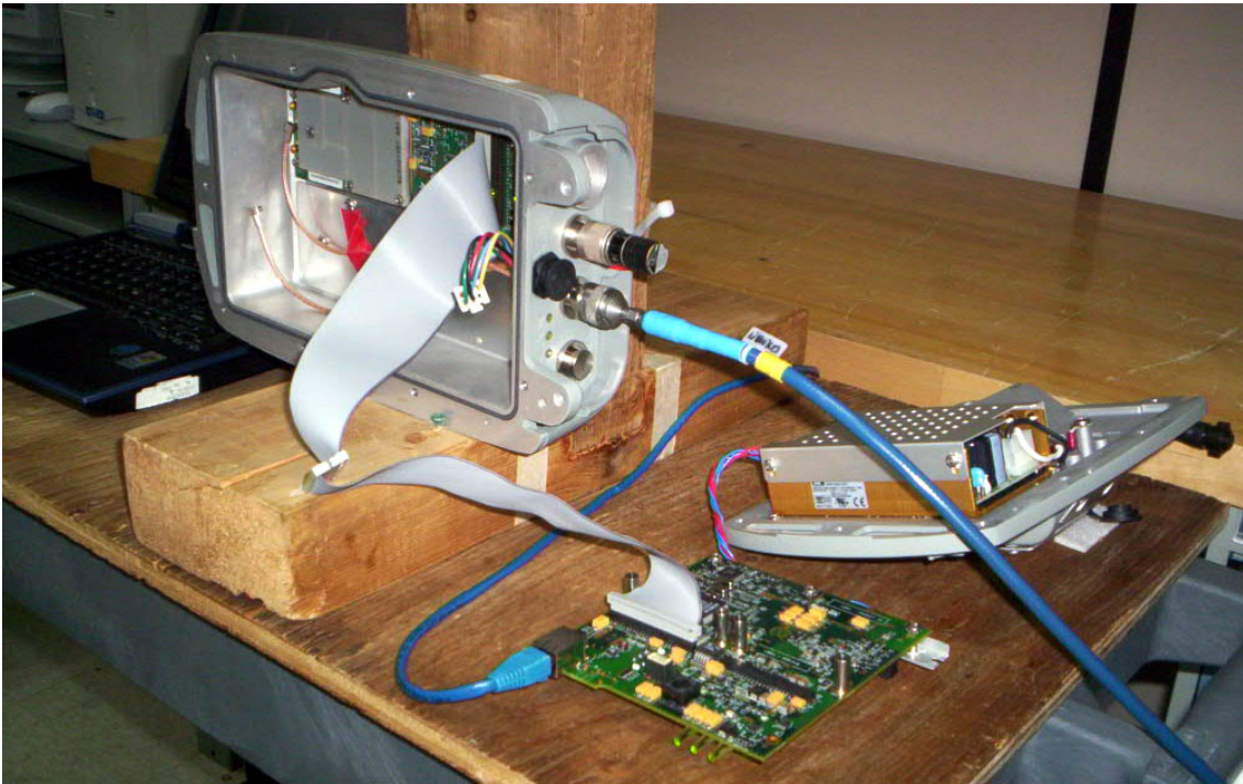
Module connected to host
