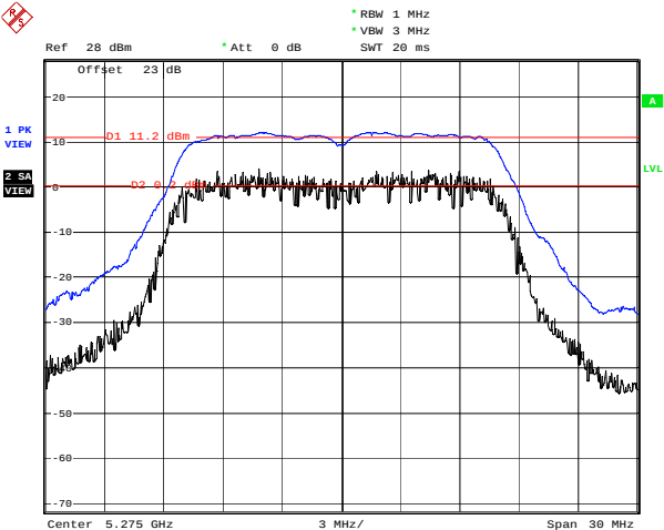
6Mb/s---5275MHz
