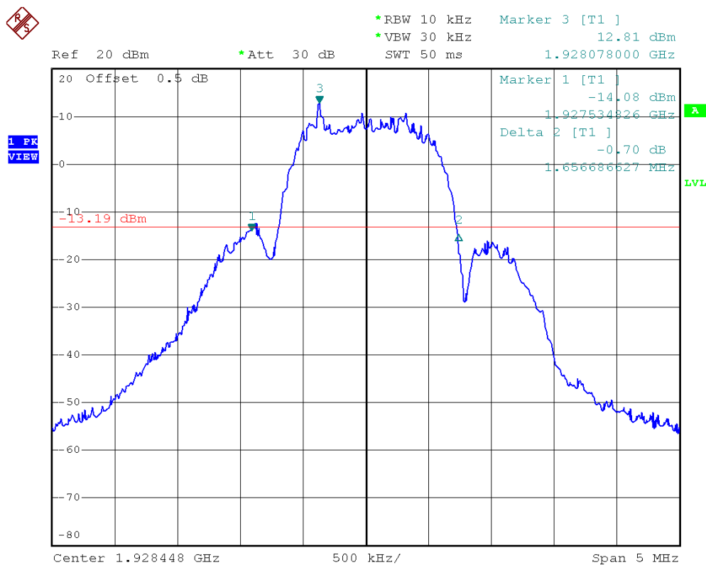
Plot 1D. Highest Channel 26dB Emission Bandwidth (Traffic Carrier)
