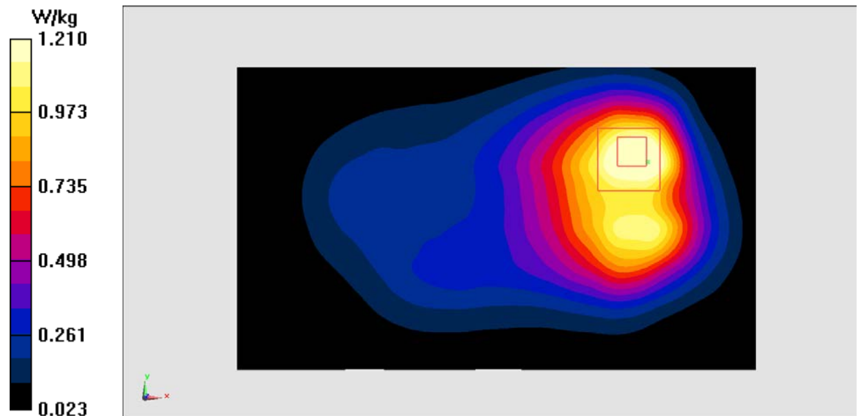
Fig.18 1700 MHz
