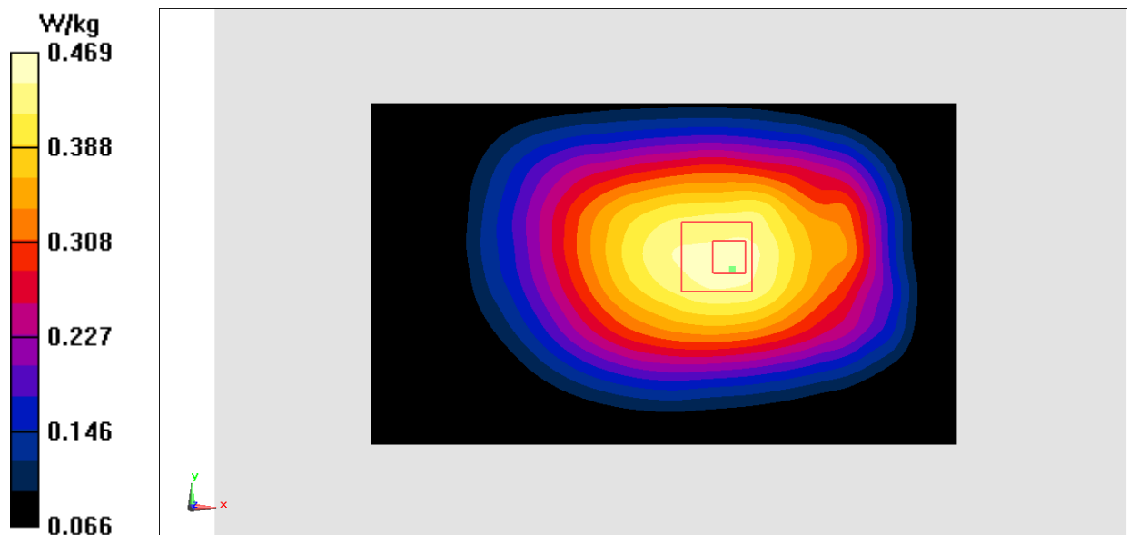
Fig.24 LTE Band17
