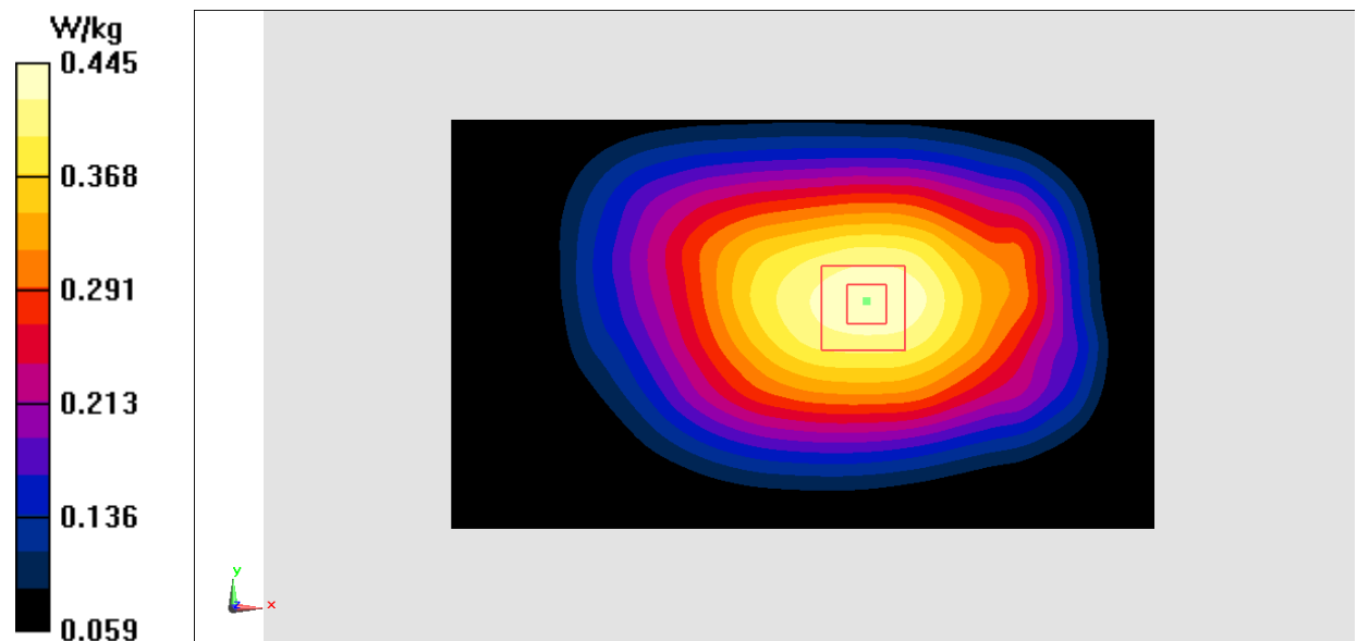
Fig.22 LTE Band12
