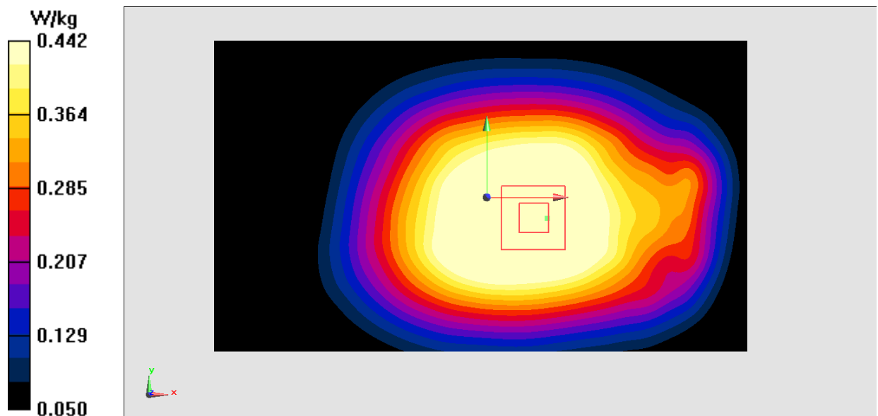
Fig.20 LTE Band5
