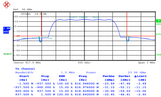
Lower Band Edge Plot on Channel 476 (817.9MHz)
