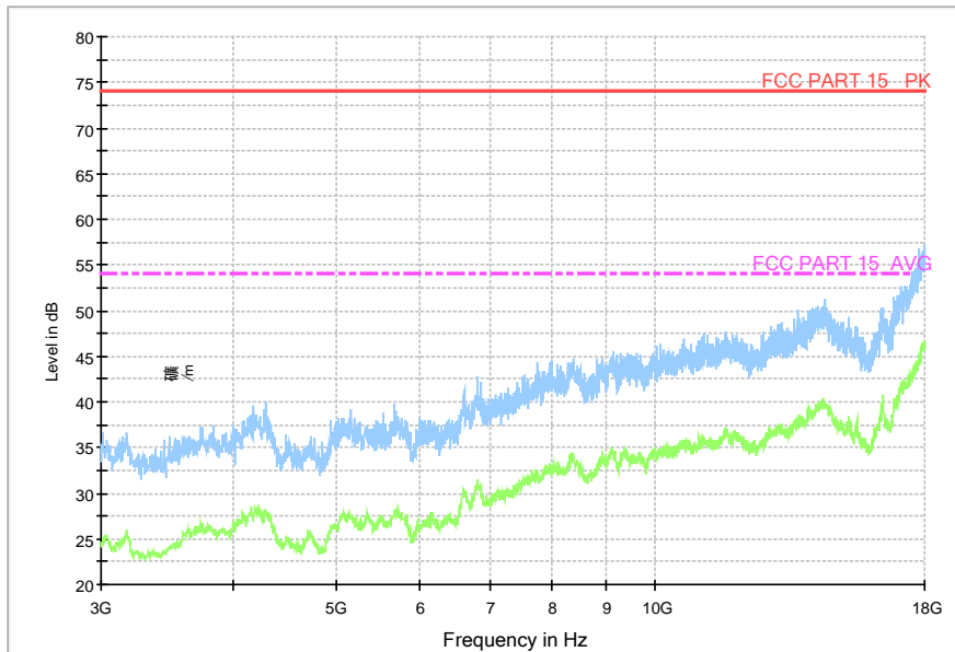
Normal RE_3G-18GHz_filter
