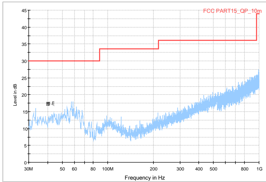
Normal RE_30M-1GHz_10m
