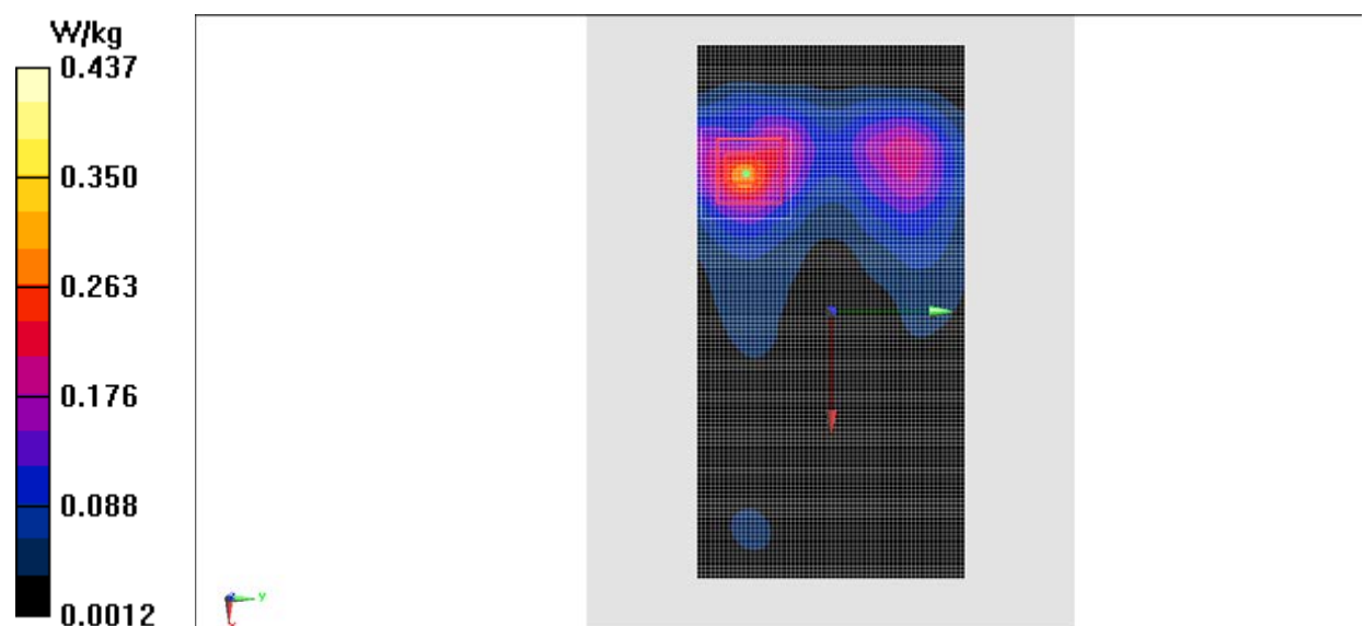
Fig.16 2450 MHz
