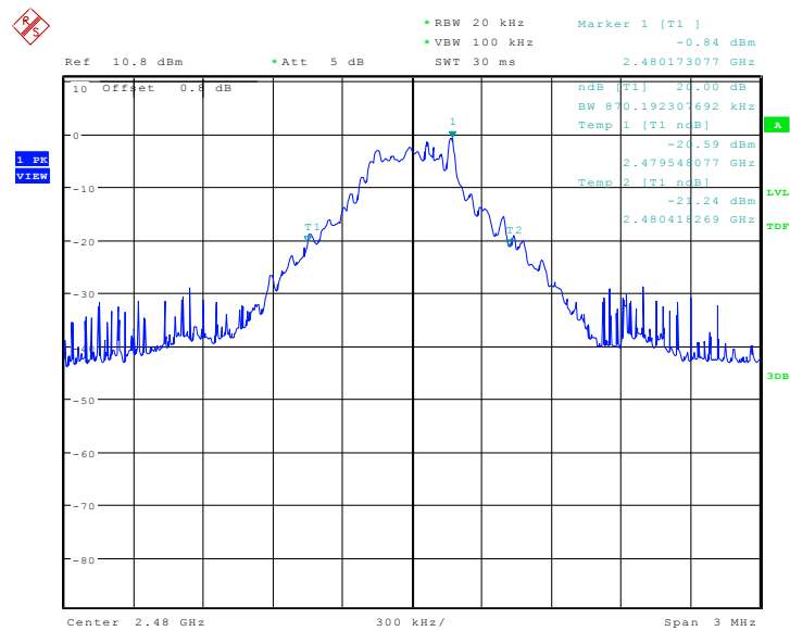
Fig.71. 20dB Bandwidth: GFSK, Channel 39
