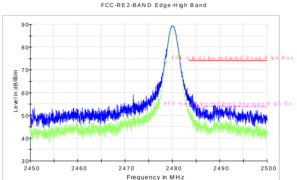
Fig.47. Radiated emission (Power) GFSK, high channel
