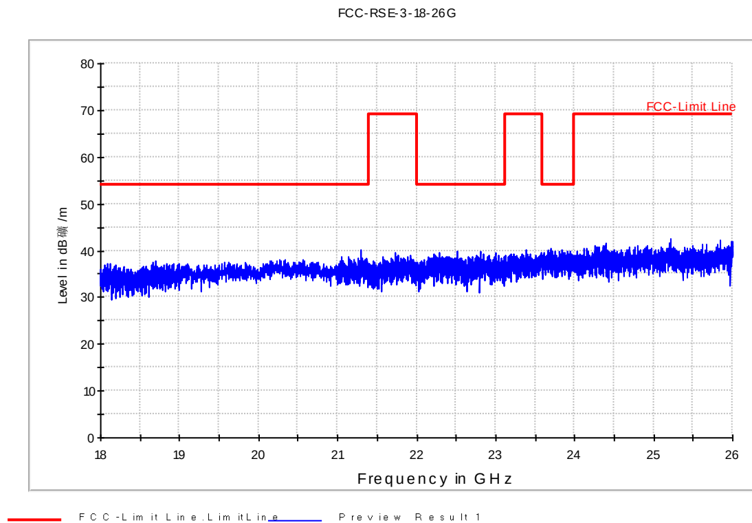
Fig.48. Radiated emission: GFSK, 18 GHz - 26 GHz
