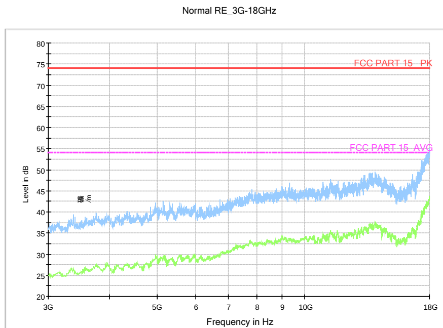
Fig.82. Radiated emission: 8DPSK, Channel 39, 3 GHz - 18 GHz
