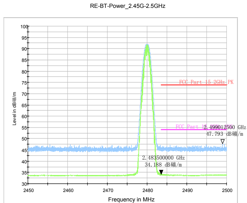
Fig.67. Radiated emission (Power) GFSK, high channel
