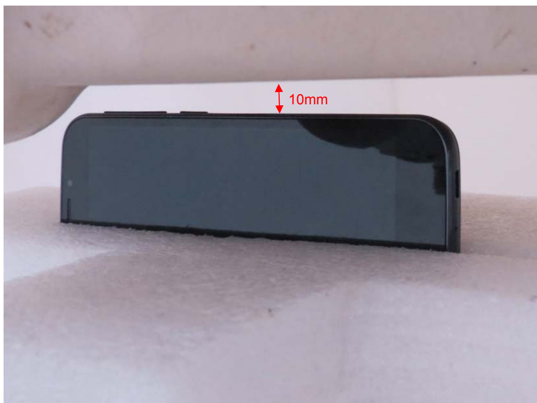
Picture 18: Right Edge, the distance from handset to the bottom of the Phantom is 10mm
